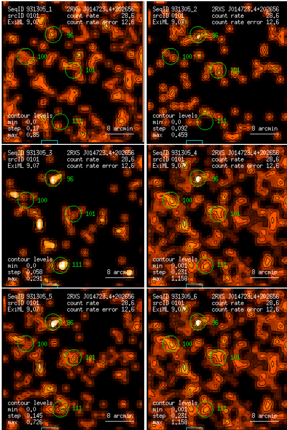
Figure 101: RASS 931305: detection 0101: band rate images, Gaussian filter: (1) PSPC channels 11 – 41, (2) 52 – 90, (3) 91 – 201, (4) 11 – 235, (5) 52 – 201, (6) 11 – 201. Broad band rates in counts/ks. Band rate contour levels in counts/ks/arcmin 2 .
