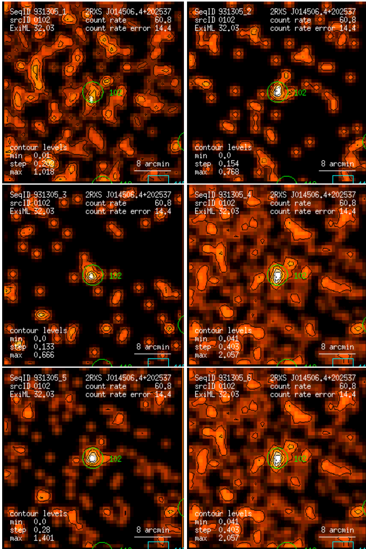
Figure 102: RASS 931305: detection 0102: band rate images, Gaussian filter: (1) PSPC channels 11 – 41, (2) 52 – 90, (3) 91 – 201, (4) 11 – 235, (5) 52 – 201, (6) 11 – 201. Broad band rates in counts/ks. Band rate contour levels in counts/ks/arcmin 2 .
