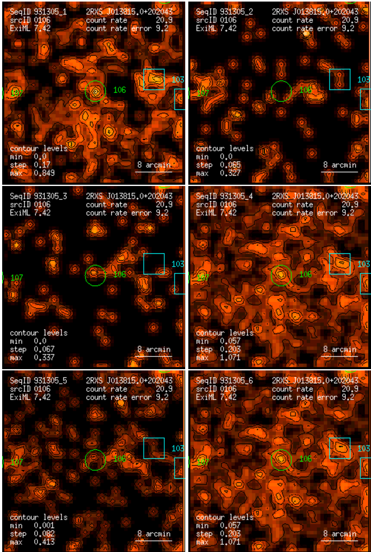
Figure 106: RASS 931305: detection 0106: band rate images, Gaussian filter: (1) PSPC channels 11 – 41, (2) 52 – 90, (3) 91 – 201, (4) 11 – 235, (5) 52 – 201, (6) 11 – 201. Broad band rates in counts/ks. Band rate contour levels in counts/ks/arcmin 2 .
