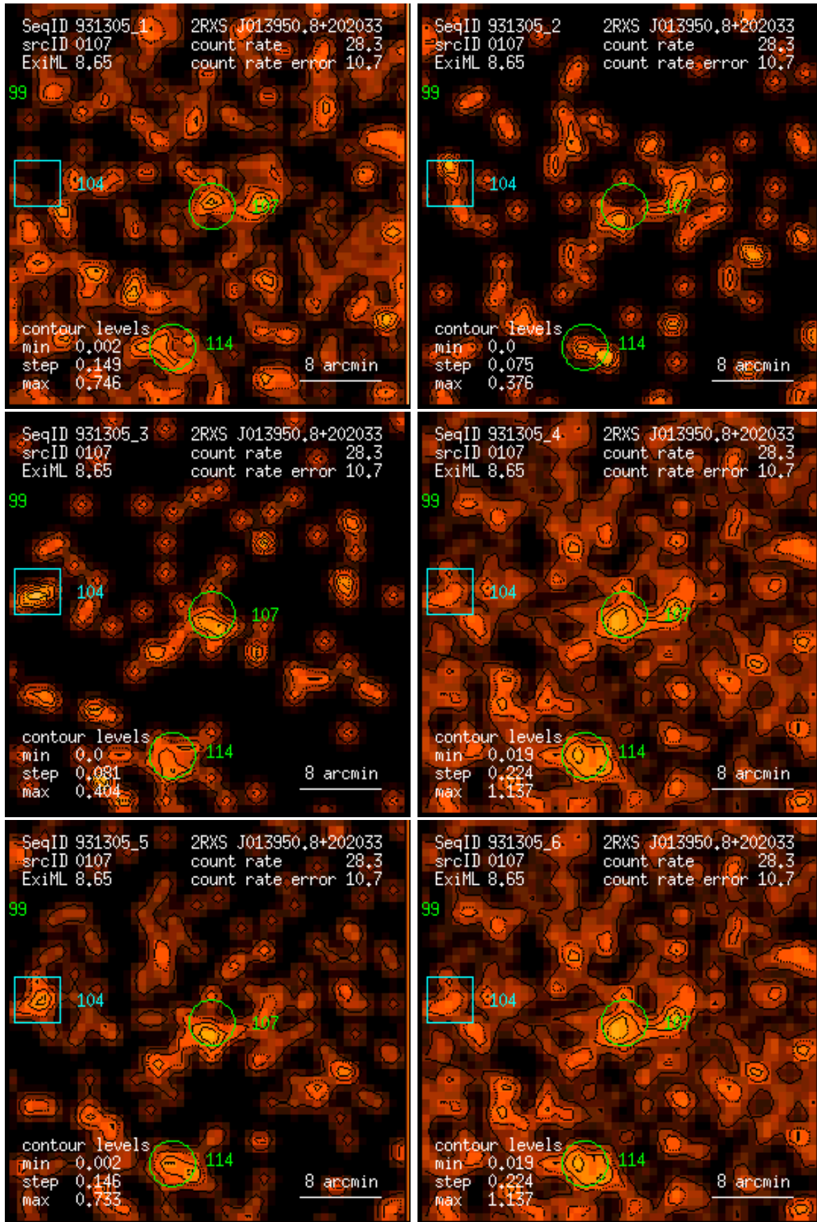
Figure 107: RASS 931305: detection 0107: band rate images, Gaussian filter: (1) PSPC channels 11 – 41, (2) 52 – 90, (3) 91 – 201, (4) 11 – 235, (5) 52 – 201, (6) 11 – 201. Broad band rates in counts/ks. Band rate contour levels in counts/ks/arcmin 2 .
