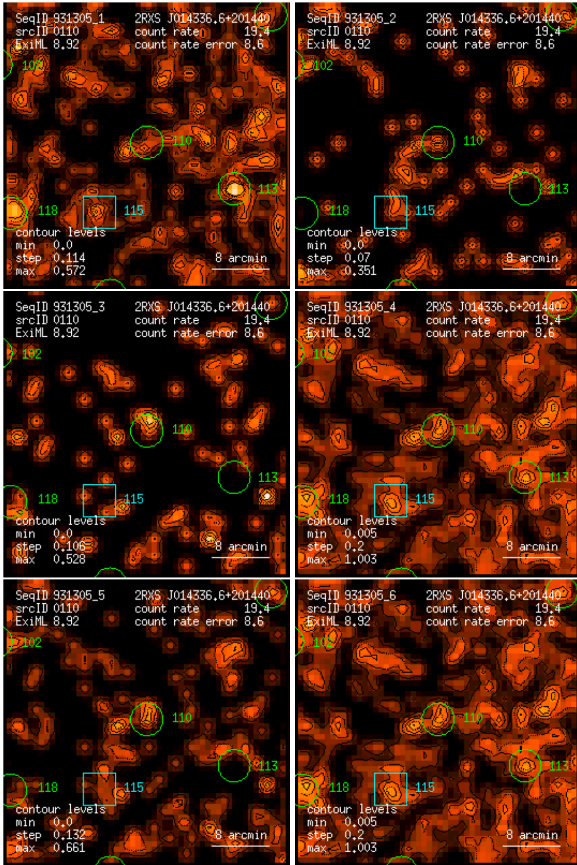
Figure 110: RASS 931305: detection 0110: band rate images, Gaussian filter: (1) PSPC channels 11 – 41, (2) 52 – 90, (3) 91 – 201, (4) 11 – 235, (5) 52 – 201, (6) 11 – 201. Broad band rates in counts/ks. Band rate contour levels in counts/ks/arcmin 2 .
