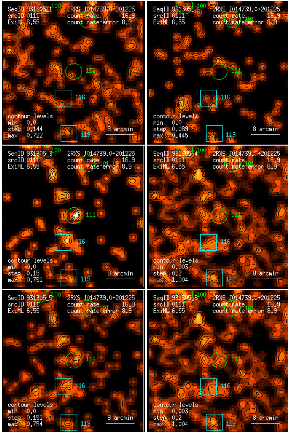
Figure 111: RASS 931305: detection 0111: band rate images, Gaussian filter: (1) PSPC channels 11 – 41, (2) 52 – 90, (3) 91 – 201, (4) 11 – 235, (5) 52 – 201, (6) 11 – 201. Broad band rates in counts/ks. Band rate contour levels in counts/ks/arcmin 2 .
