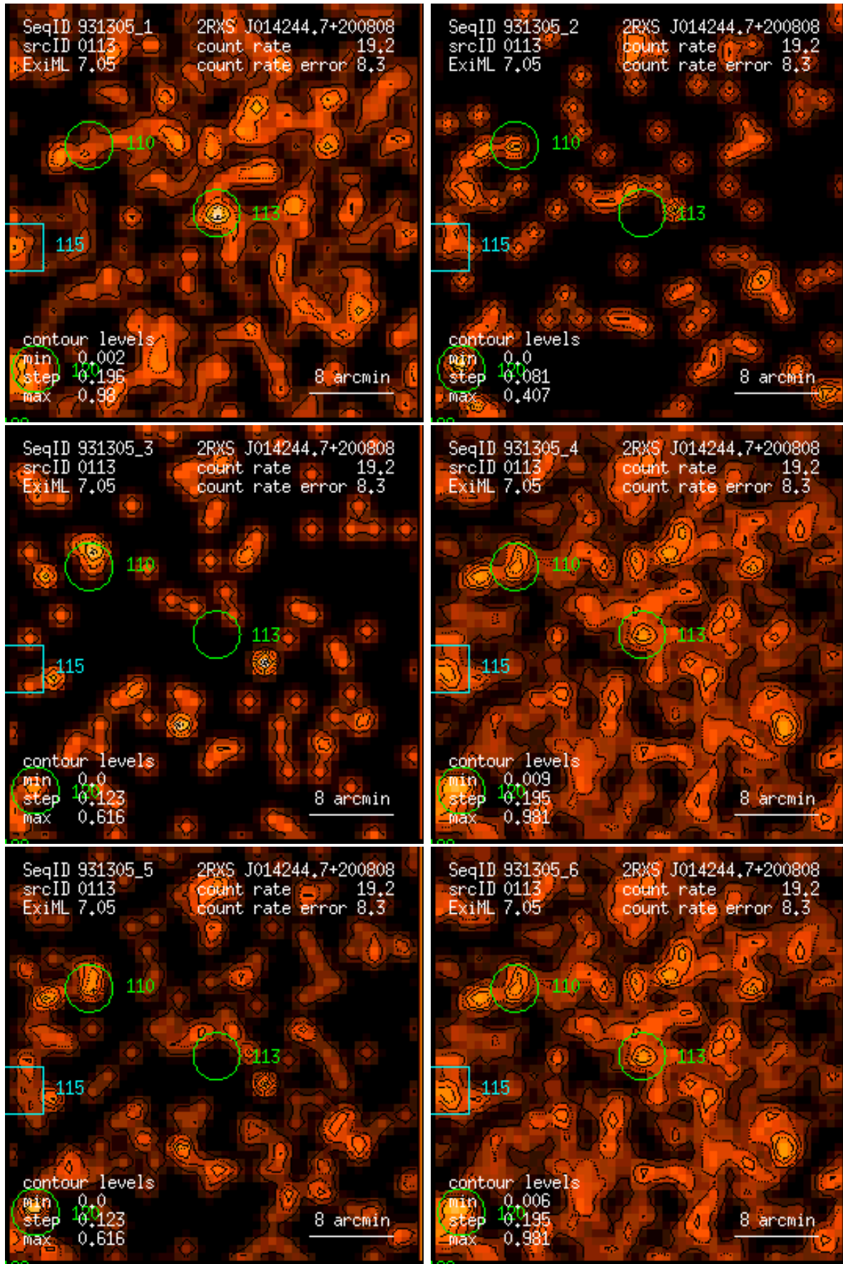
Figure 113: RASS 931305: detection 0113: band rate images, Gaussian filter: (1) PSPC channels 11 – 41, (2) 52 – 90, (3) 91 – 201, (4) 11 – 235, (5) 52 – 201, (6) 11 – 201. Broad band rates in counts/ks. Band rate contour levels in counts/ks/arcmin 2 .
