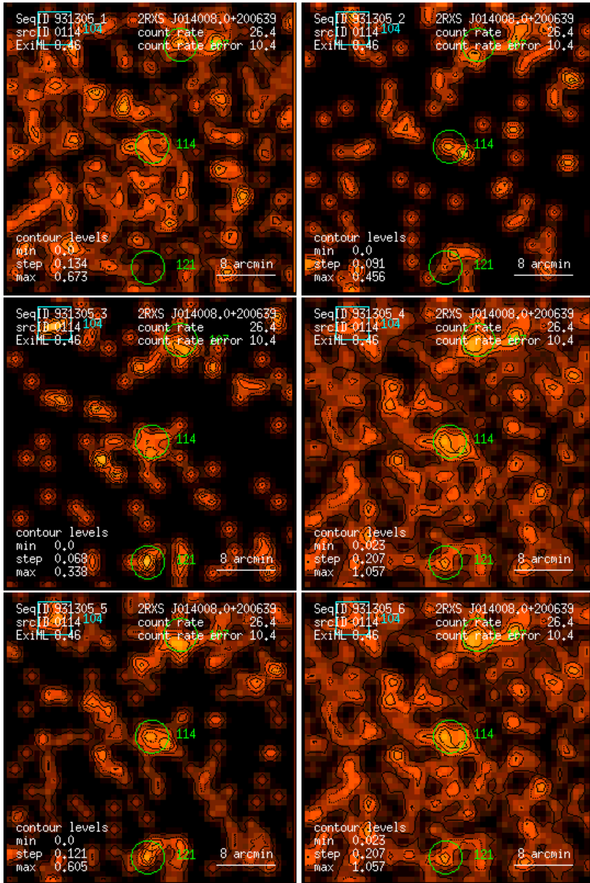
Figure 114: RASS 931305: detection 0114: band rate images, Gaussian filter: (1) PSPC channels 11 – 41, (2) 52 – 90, (3) 91 – 201, (4) 11 – 235, (5) 52 – 201, (6) 11 – 201. Broad band rates in counts/ks. Band rate contour levels in counts/ks/arcmin 2 .
