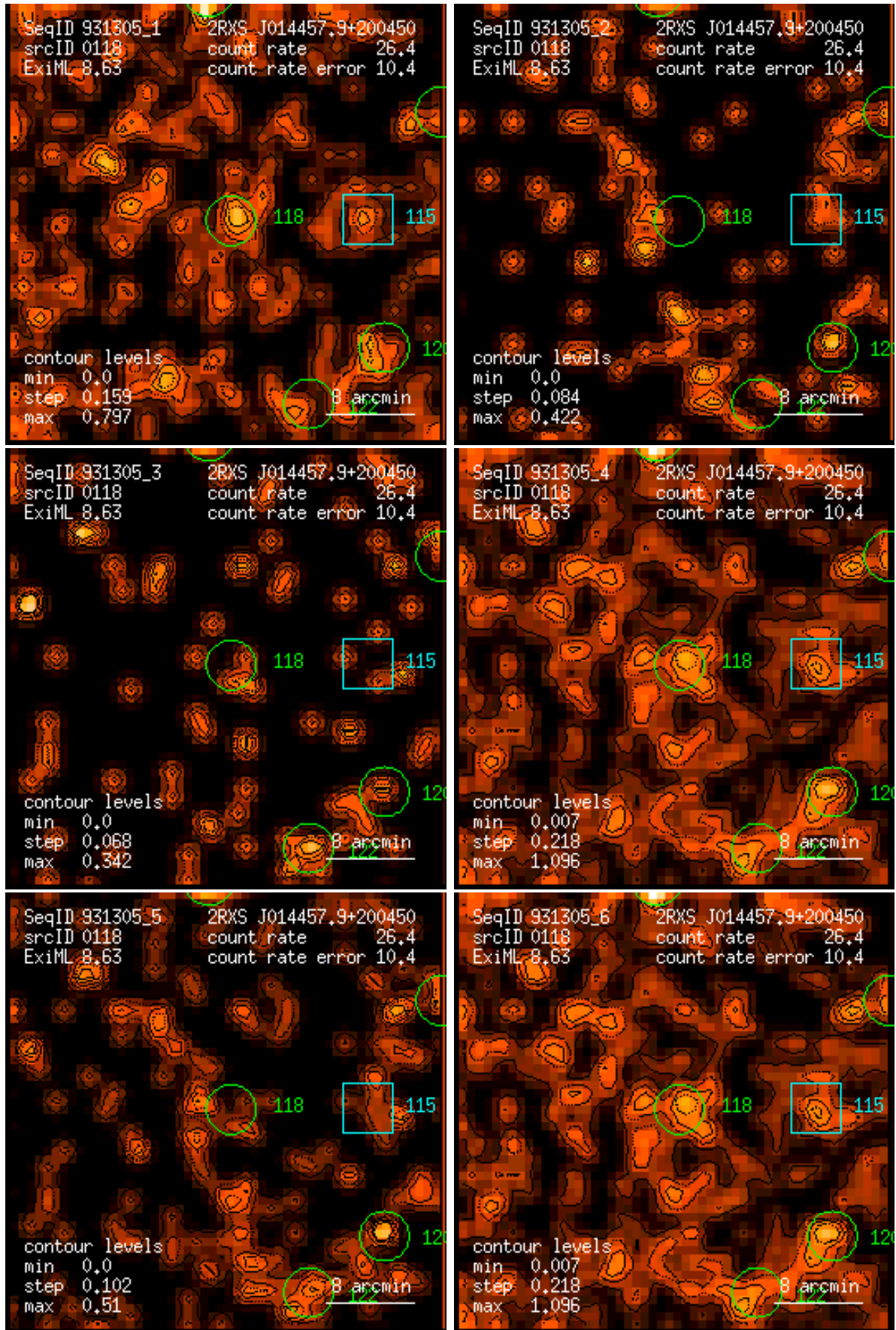
Figure 118: RASS 931305: detection 0118: band rate images, Gaussian filter: (1) PSPC channels 11 – 41, (2) 52 – 90, (3) 91 – 201, (4) 11 – 235, (5) 52 – 201, (6) 11 – 201. Broad band rates in counts/ks. Band rate contour levels in counts/ks/arcmin 2 .
