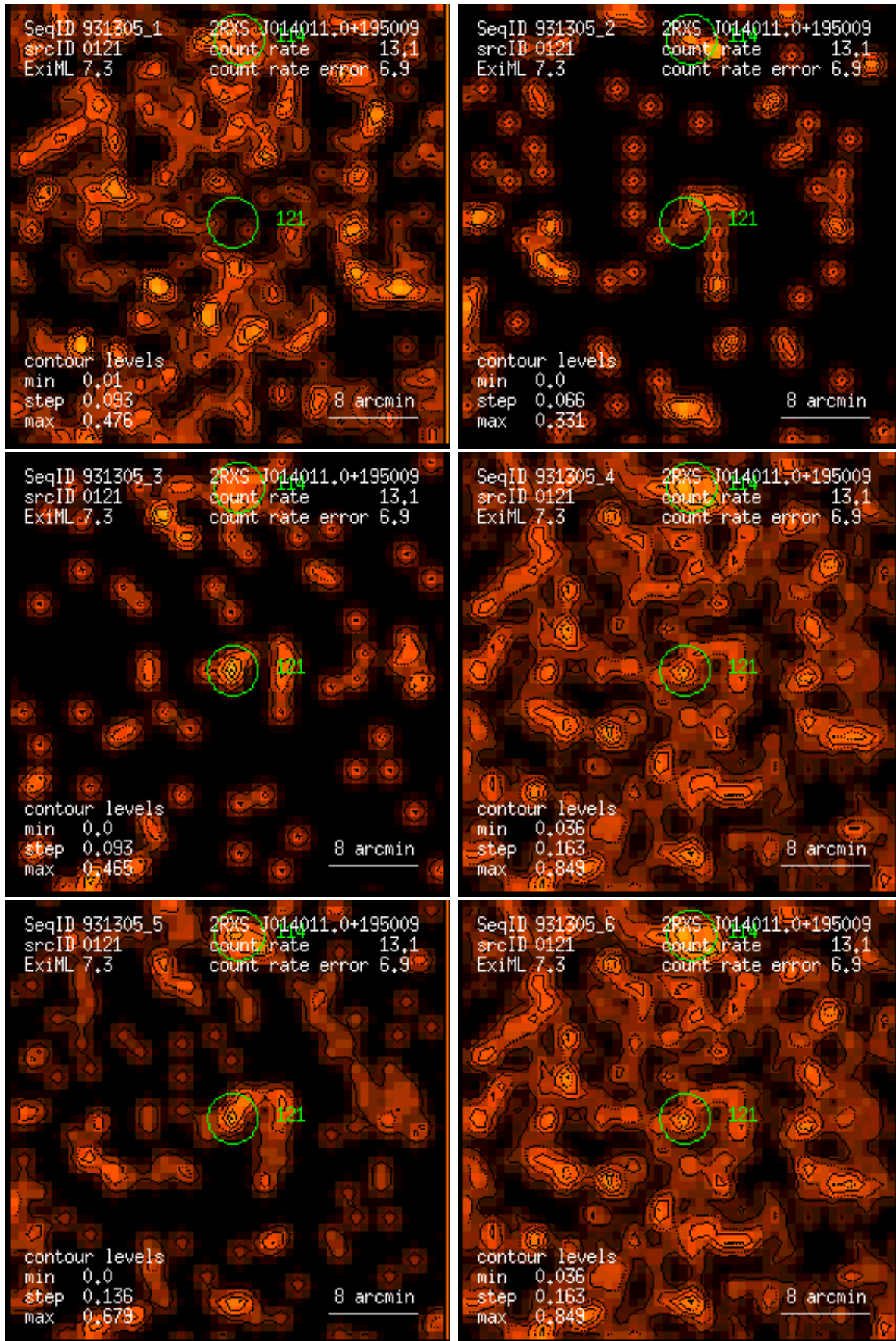
Figure 121: RASS 931305: detection 0121: band rate images, Gaussian filter: (1) PSPC channels 11 – 41, (2) 52 – 90, (3) 91 – 201, (4) 11 – 235, (5) 52 – 201, (6) 11 – 201. Broad band rates in counts/ks. Band rate contour levels in counts/ks/arcmin 2 .
