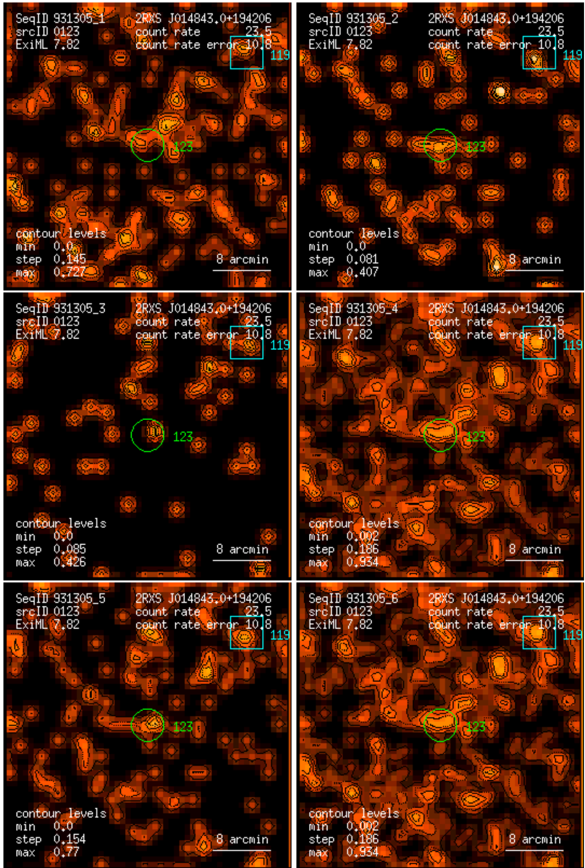
Figure 123: RASS 931305: detection 0123: band rate images, Gaussian filter: (1) PSPC channels 11 – 41, (2) 52 – 90, (3) 91 – 201, (4) 11 – 235, (5) 52 – 201, (6) 11 – 201. Broad band rates in counts/ks. Band rate contour levels in counts/ks/arcmin 2 .
