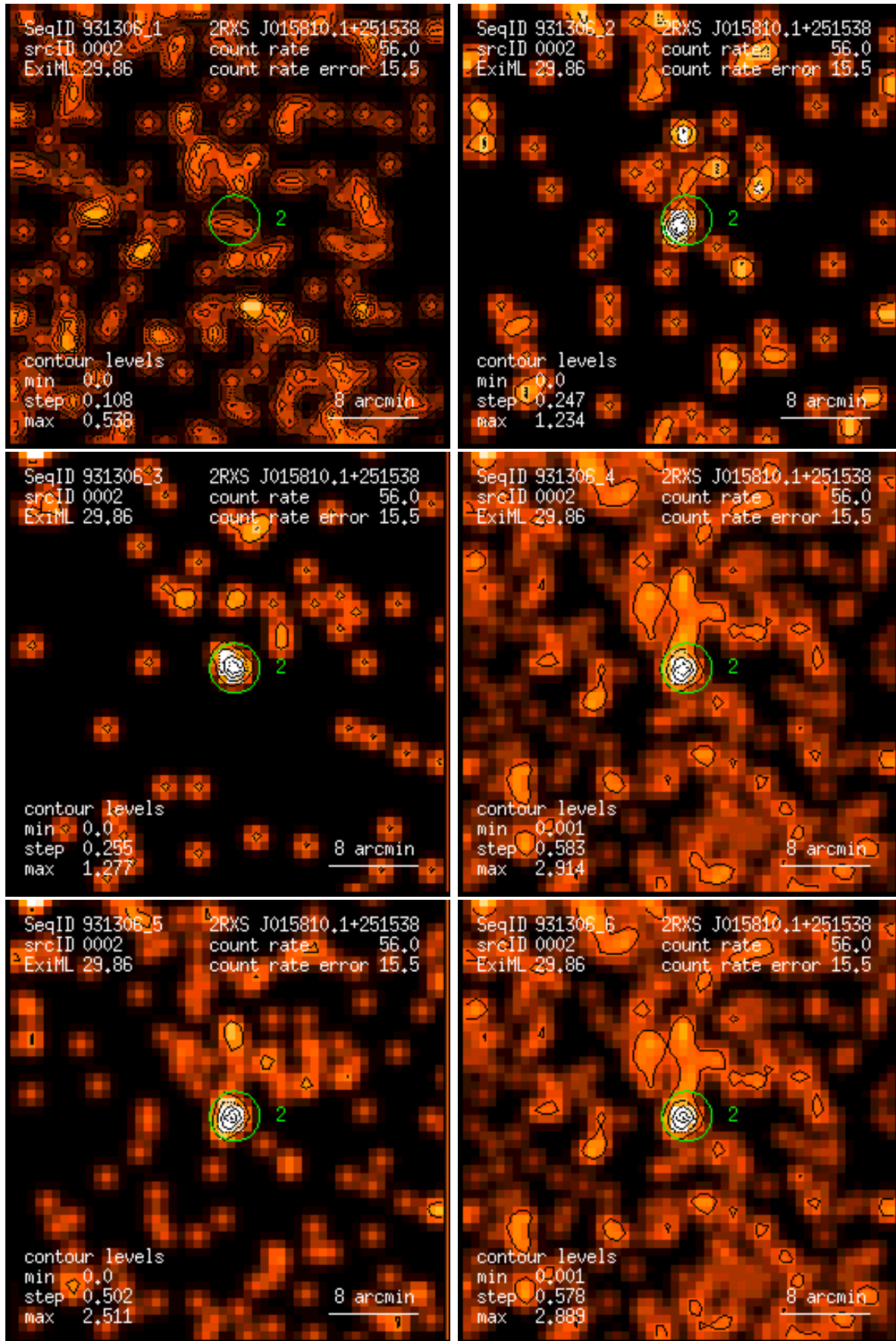
Figure 2: RASS 931306: detection 0002: band rate images, Gaussian filter: (1) PSPC channels 11 – 41, (2) 52 – 90, (3) 91 – 201, (4) 11 – 235, (5) 52 – 201, (6) 11 – 201. Broad band rates in counts/ks. Band rate contour levels in counts/ks/arcmin 2 .
