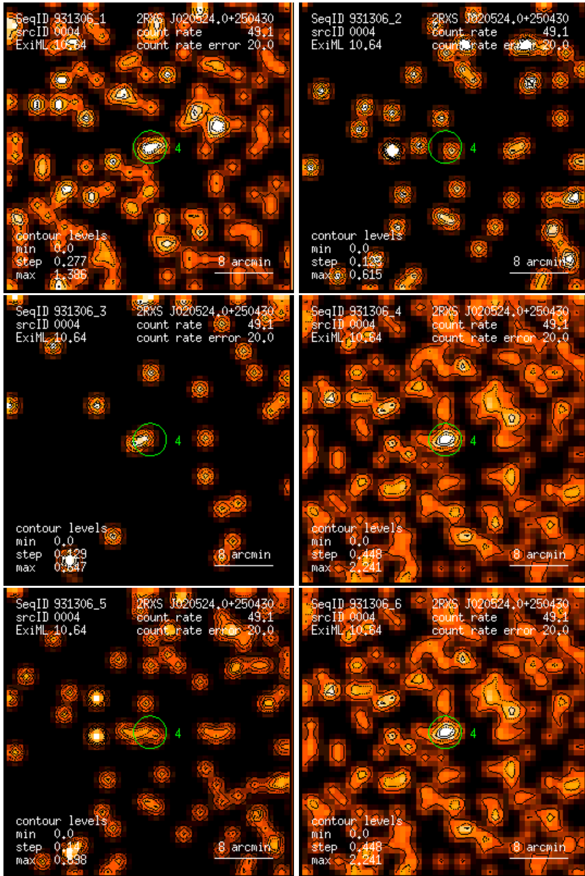
Figure 4: RASS 931306: detection 0004: band rate images, Gaussian filter: (1) PSPC channels 11 – 41, (2) 52 – 90, (3) 91 – 201, (4) 11 – 235, (5) 52 – 201, (6) 11 – 201. Broad band rates in counts/ks. Band rate contour levels in counts/ks/arcmin 2 .
