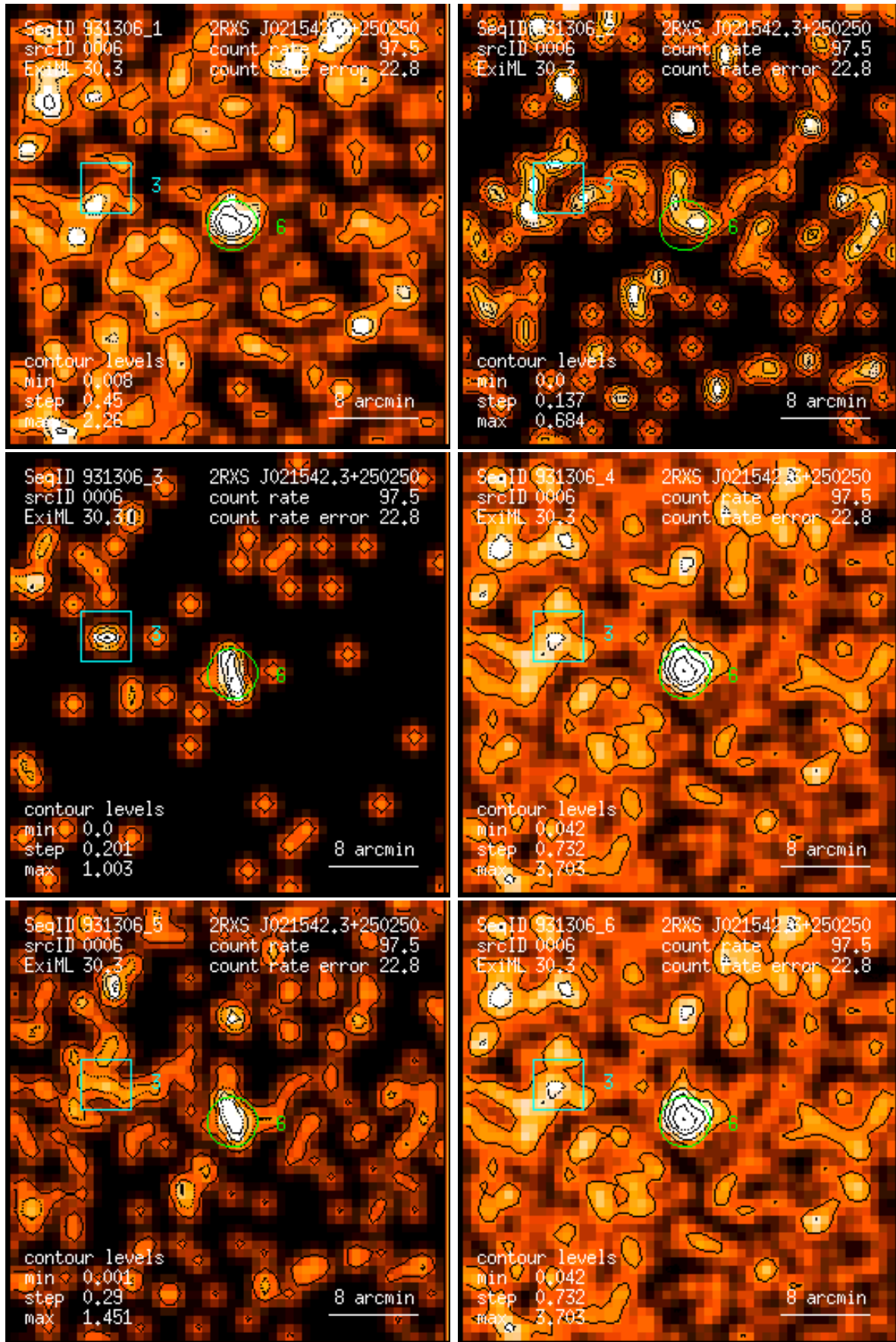
Figure 6: RASS 931306: detection 0006: band rate images, Gaussian filter: (1) PSPC channels 11 – 41, (2) 52 – 90, (3) 91 – 201, (4) 11 – 235, (5) 52 – 201, (6) 11 – 201. Broad band rates in counts/ks. Band rate contour levels in counts/ks/arcmin 2 .
