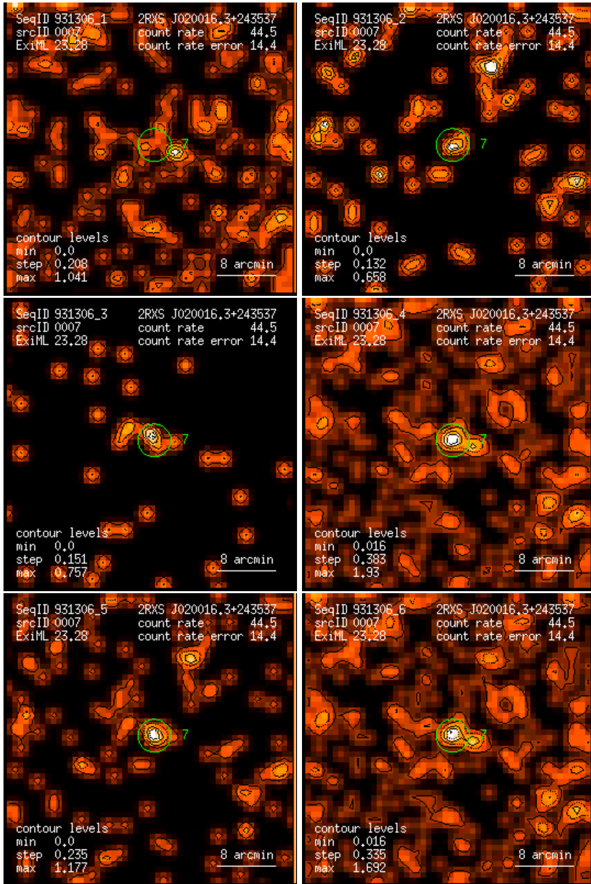
Figure 7: RASS 931306: detection 0007: band rate images, Gaussian filter: (1) PSPC channels 11 – 41, (2) 52 – 90, (3) 91 – 201, (4) 11 – 235, (5) 52 – 201, (6) 11 – 201. Broad band rates in counts/ks. Band rate contour levels in counts/ks/arcmin 2 .
