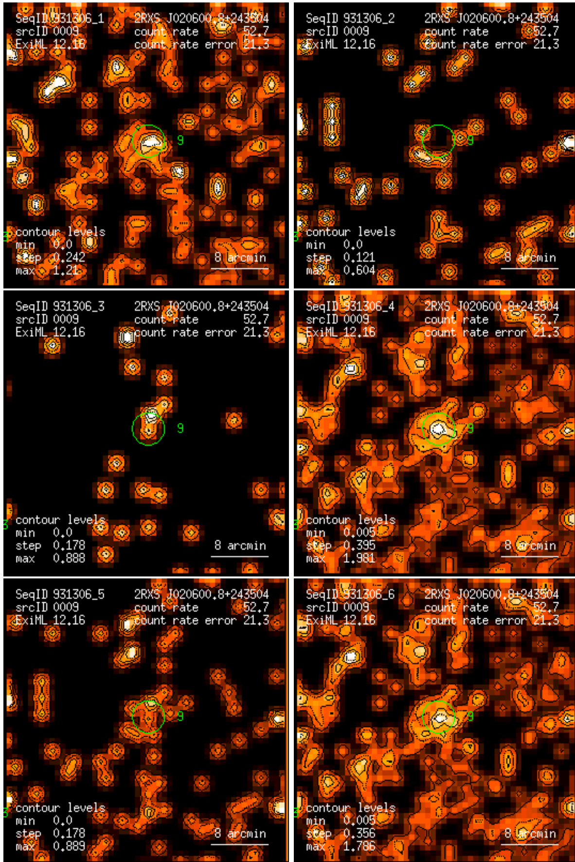
Figure 9: RASS 931306: detection 0009: band rate images, Gaussian filter: (1) PSPC channels 11 – 41, (2) 52 – 90, (3) 91 – 201, (4) 11 – 235, (5) 52 – 201, (6) 11 – 201. Broad band rates in counts/ks. Band rate contour levels in counts/ks/arcmin 2 .
