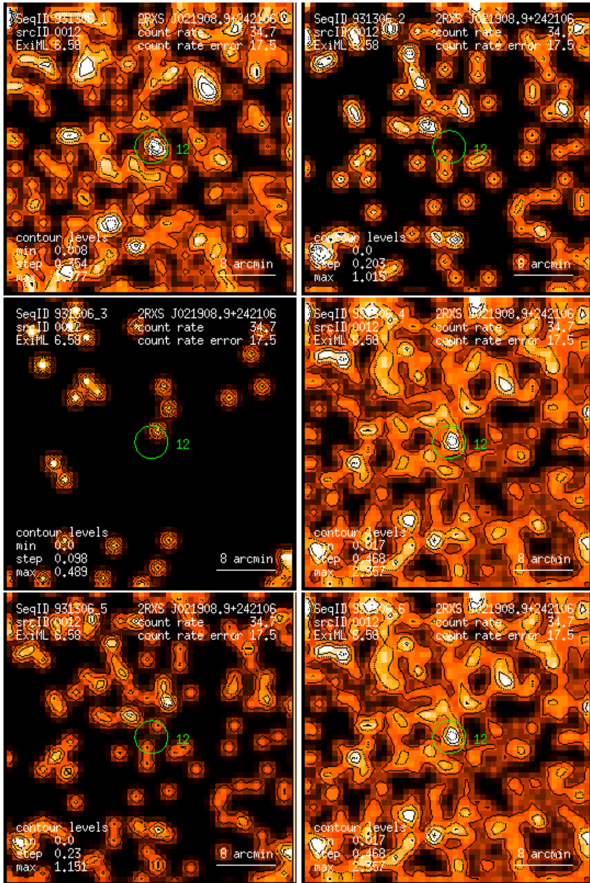
Figure 12: RASS 931306: detection 0012: band rate images, Gaussian filter: (1) PSPC channels 11 – 41, (2) 52 – 90, (3) 91 – 201, (4) 11 – 235, (5) 52 – 201, (6) 11 – 201. Broad band rates in counts/ks. Band rate contour levels in counts/ks/arcmin 2 .
