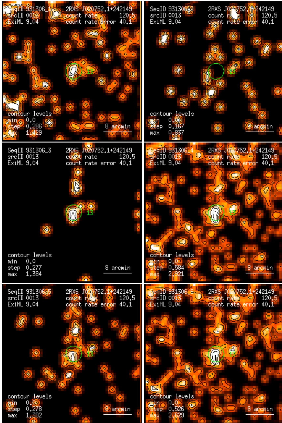
Figure 13: RASS 931306: detection 0013: band rate images, Gaussian filter: (1) PSPC channels 11 – 41, (2) 52 – 90, (3) 91 – 201, (4) 11 – 235, (5) 52 – 201, (6) 11 – 201. Broad band rates in counts/ks. Band rate contour levels in counts/ks/arcmin 2 .
