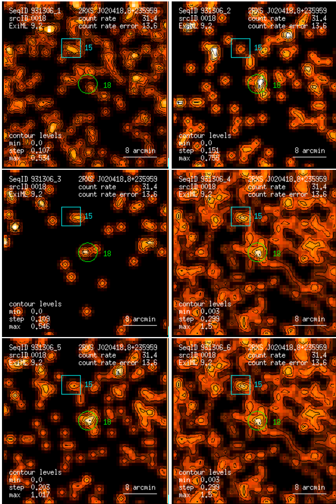
Figure 18: RASS 931306: detection 0018: band rate images, Gaussian filter: (1) PSPC channels 11 – 41, (2) 52 – 90, (3) 91 – 201, (4) 11 – 235, (5) 52 – 201, (6) 11 – 201. Broad band rates in counts/ks. Band rate contour levels in counts/ks/arcmin 2 .
