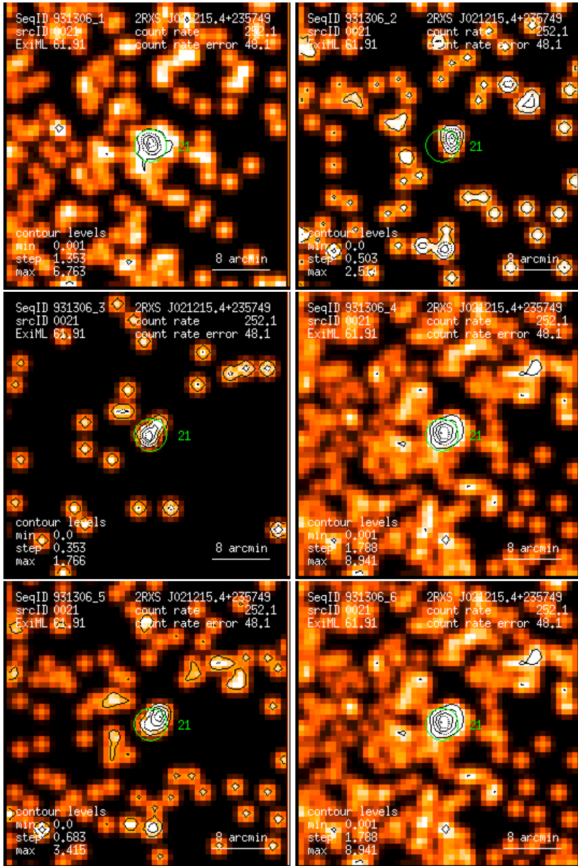
Figure 21: RASS 931306: detection 0021: band rate images, Gaussian filter: (1) PSPC channels 11 – 41, (2) 52 – 90, (3) 91 – 201, (4) 11 – 235, (5) 52 – 201, (6) 11 – 201. Broad band rates in counts/ks. Band rate contour levels in counts/ks/arcmin 2 .
