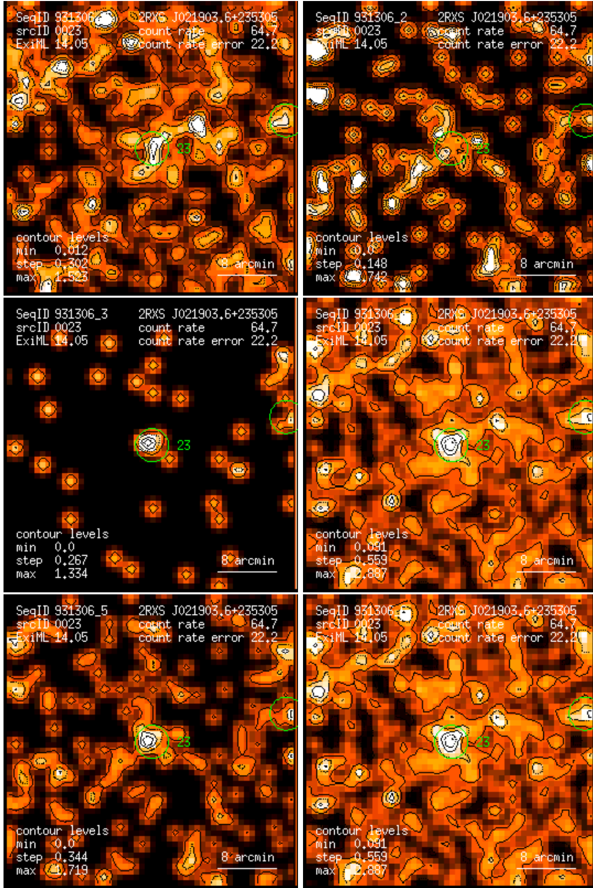
Figure 23: RASS 931306: detection 0023: band rate images, Gaussian filter: (1) PSPC channels 11 – 41, (2) 52 – 90, (3) 91 – 201, (4) 11 – 235, (5) 52 – 201, (6) 11 – 201. Broad band rates in counts/ks. Band rate contour levels in counts/ks/arcmin 2 .
