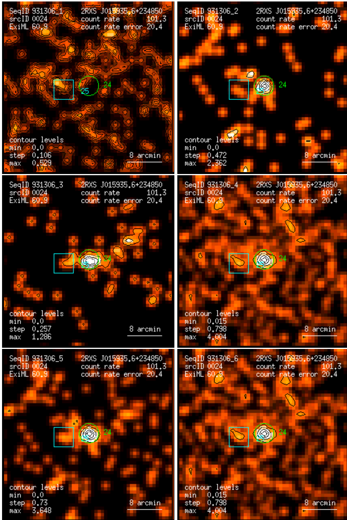
Figure 24: RASS 931306: detection 0024: band rate images, Gaussian filter: (1) PSPC channels 11 – 41, (2) 52 – 90, (3) 91 – 201, (4) 11 – 235, (5) 52 – 201, (6) 11 – 201. Broad band rates in counts/ks. Band rate contour levels in counts/ks/arcmin 2 .
