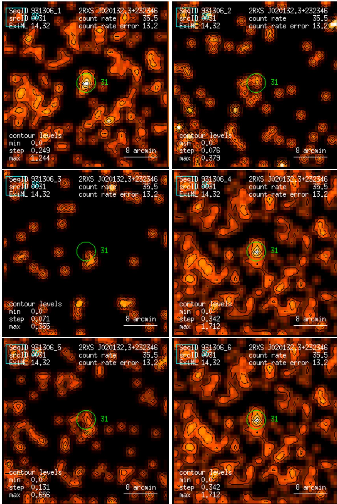
Figure 31: RASS 931306: detection 0031: band rate images, Gaussian filter: (1) PSPC channels 11 – 41, (2) 52 – 90, (3) 91 – 201, (4) 11 – 235, (5) 52 – 201, (6) 11 – 201. Broad band rates in counts/ks. Band rate contour levels in counts/ks/arcmin 2 .
