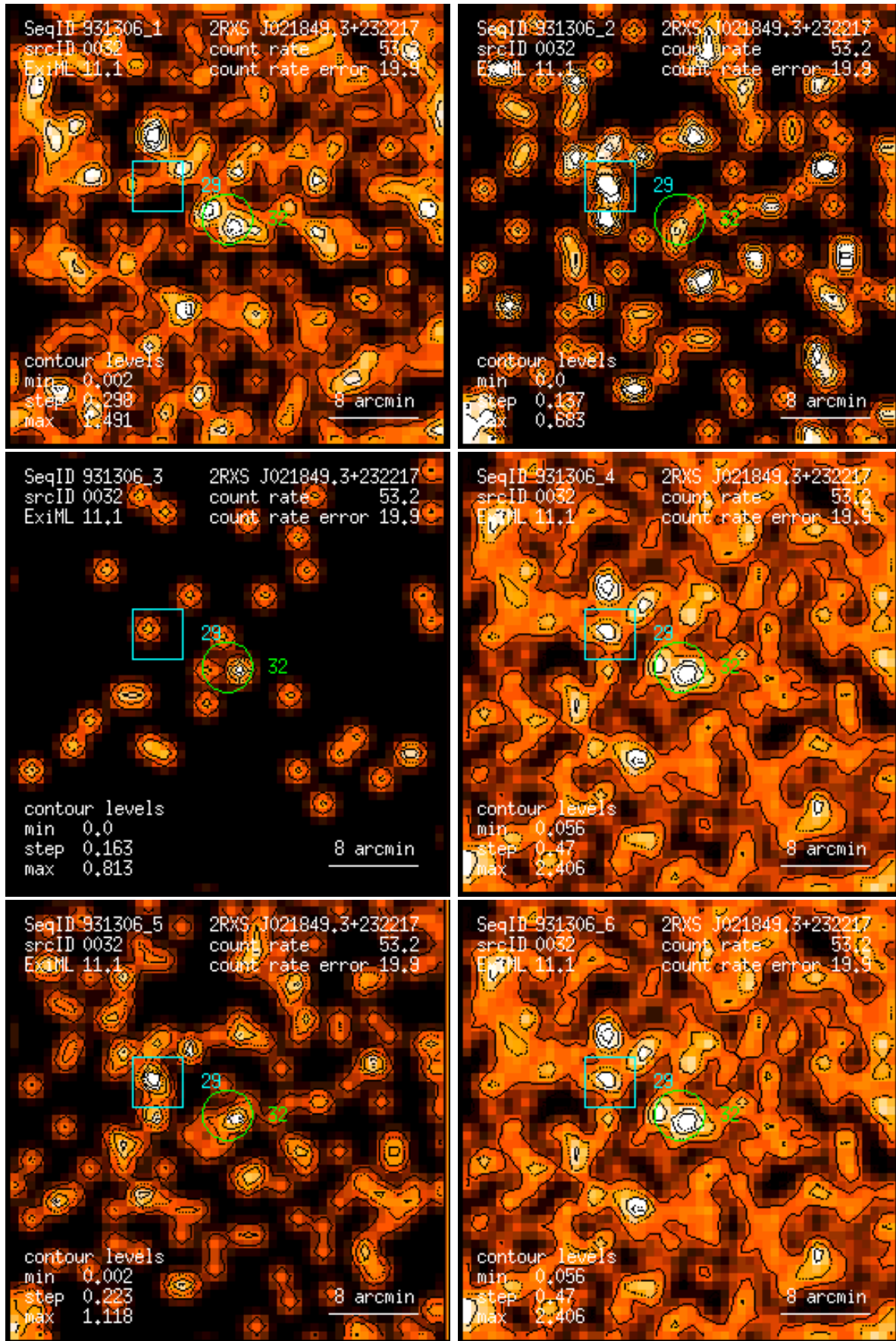
Figure 32: RASS 931306: detection 0032: band rate images, Gaussian filter: (1) PSPC channels 11 – 41, (2) 52 – 90, (3) 91 – 201, (4) 11 – 235, (5) 52 – 201, (6) 11 – 201. Broad band rates in counts/ks. Band rate contour levels in counts/ks/arcmin 2 .
