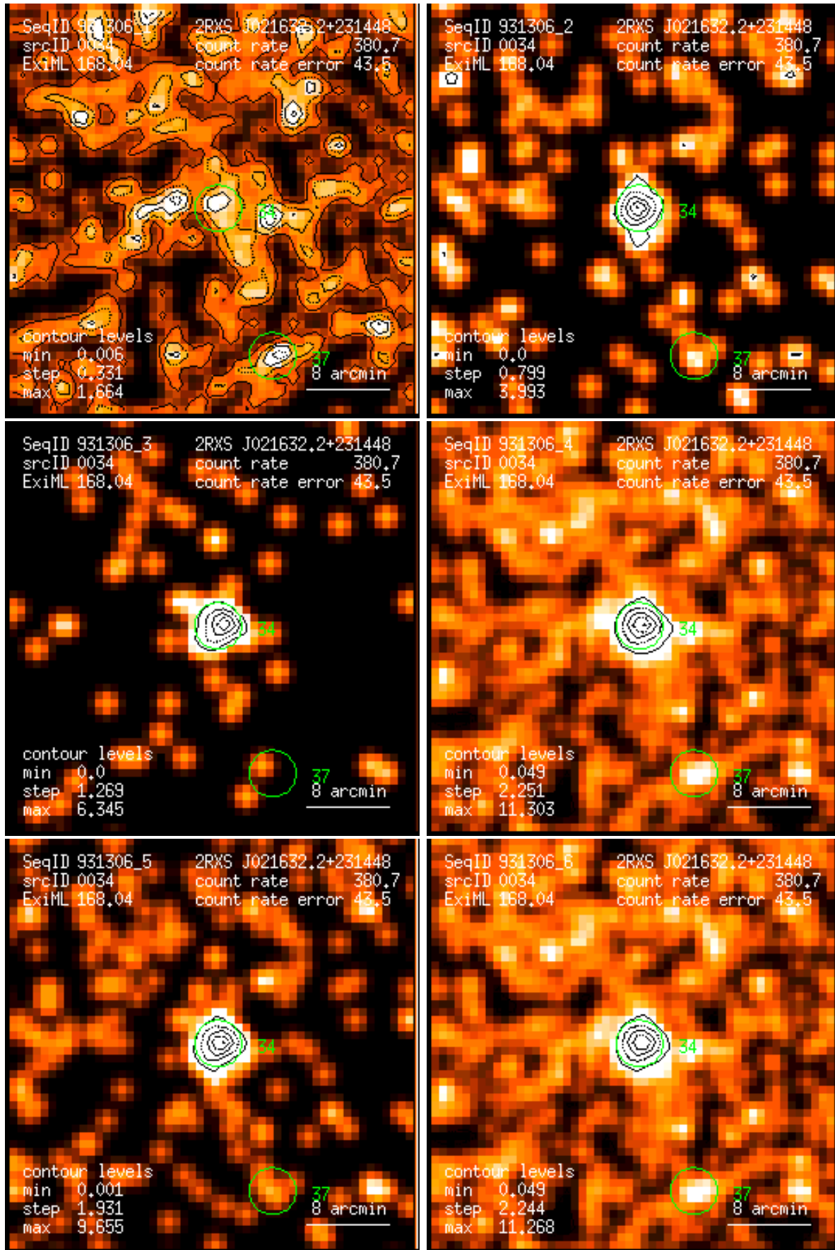
Figure 34: RASS 931306: detection 0034: band rate images, Gaussian filter: (1) PSPC channels 11 – 41, (2) 52 – 90, (3) 91 – 201, (4) 11 – 235, (5) 52 – 201, (6) 11 – 201. Broad band rates in counts/ks. Band rate contour levels in counts/ks/arcmin 2 .
