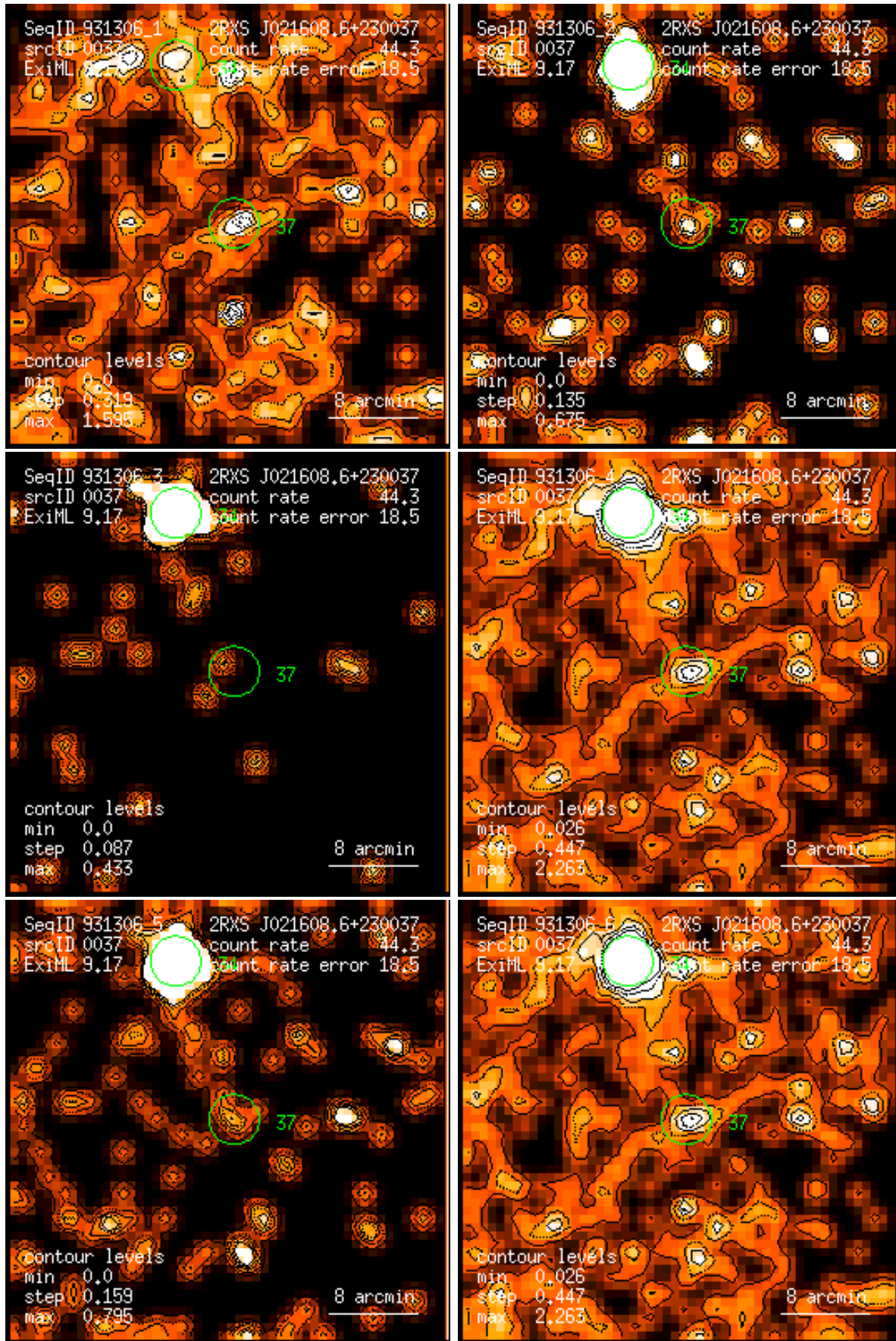
Figure 37: RASS 931306: detection 0037: band rate images, Gaussian filter: (1) PSPC channels 11 – 41, (2) 52 – 90, (3) 91 – 201, (4) 11 – 235, (5) 52 – 201, (6) 11 – 201. Broad band rates in counts/ks. Band rate contour levels in counts/ks/arcmin 2 .
