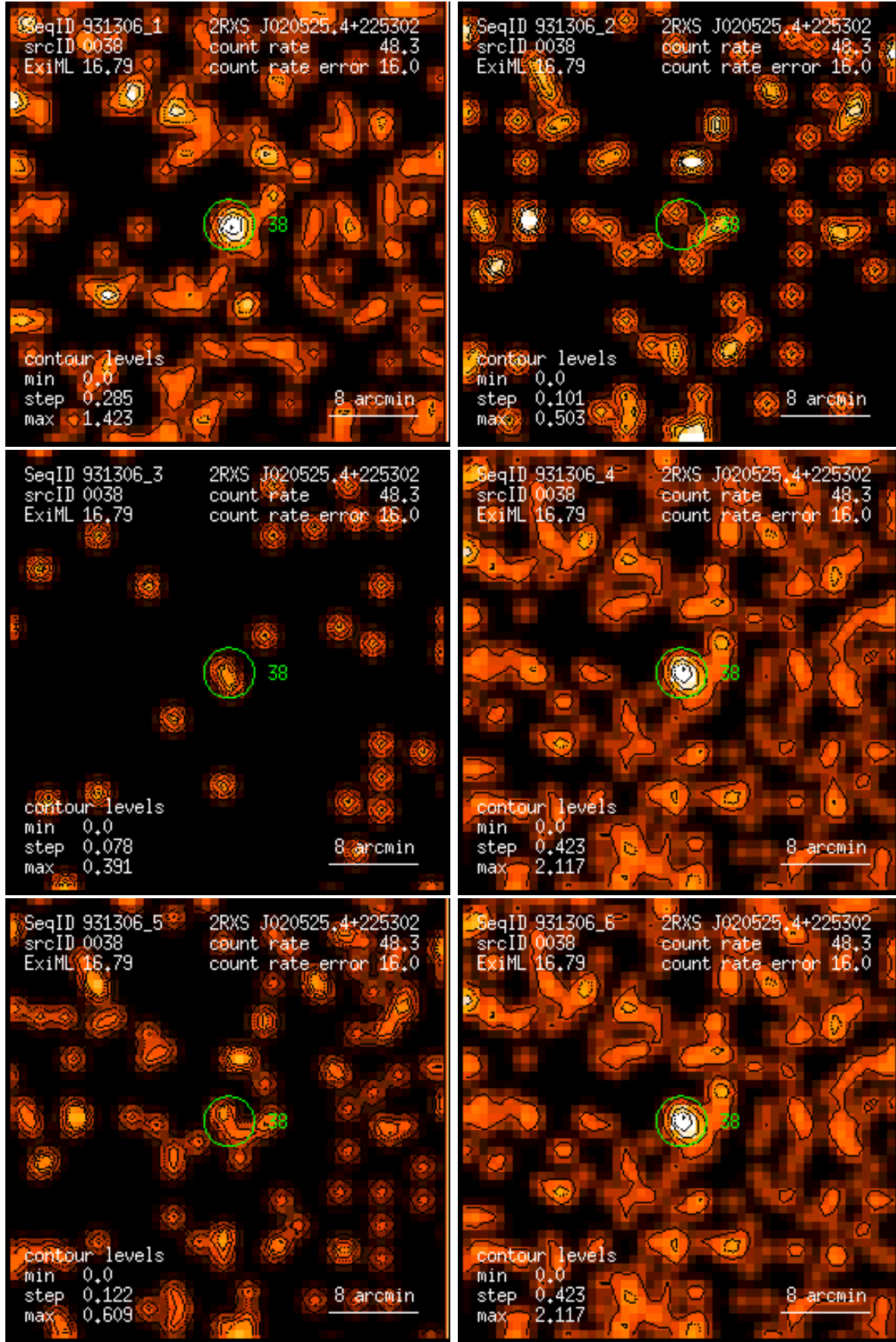
Figure 38: RASS 931306: detection 0038: band rate images, Gaussian filter: (1) PSPC channels 11 – 41, (2) 52 – 90, (3) 91 – 201, (4) 11 – 235, (5) 52 – 201, (6) 11 – 201. Broad band rates in counts/ks. Band rate contour levels in counts/ks/arcmin 2 .
