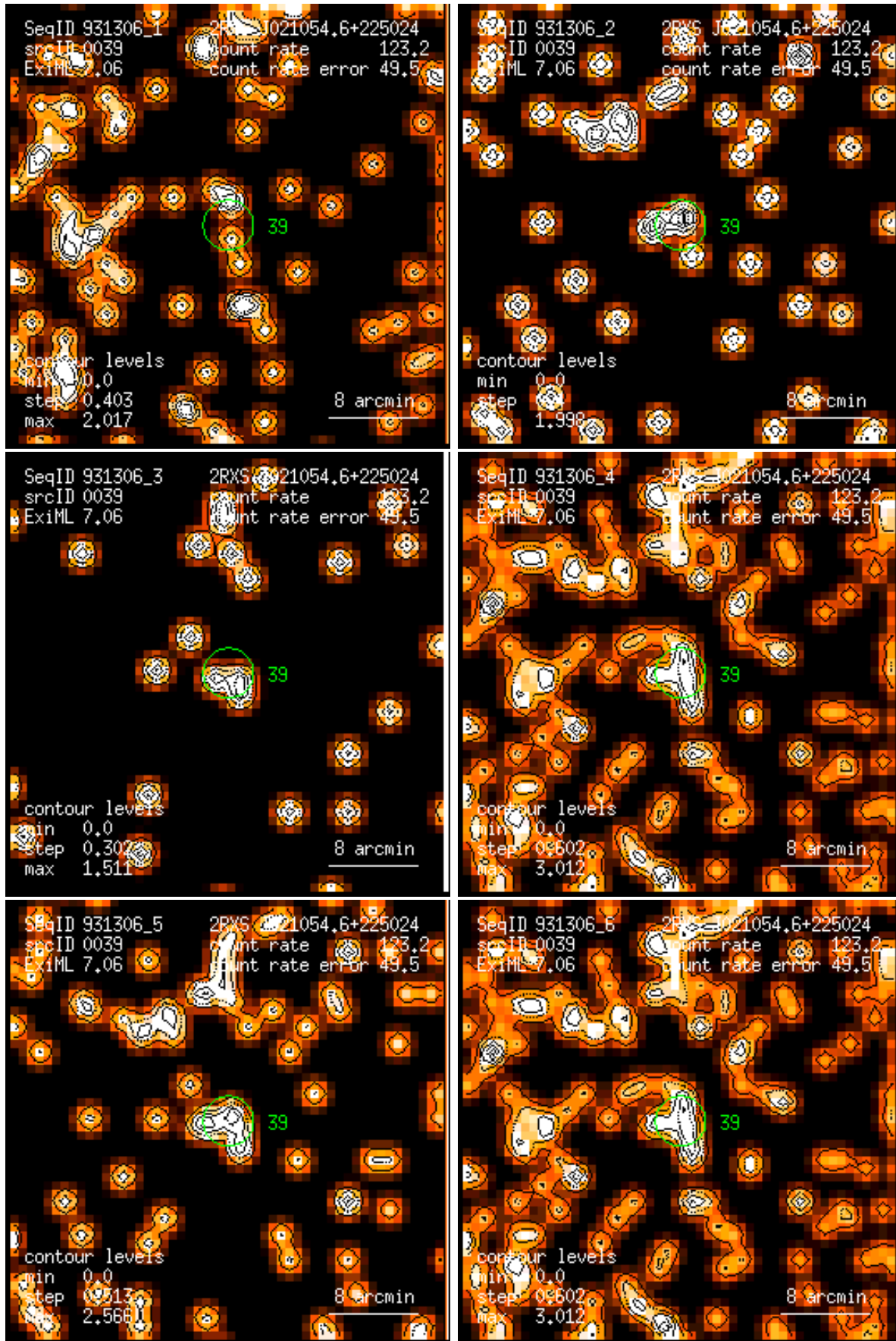
Figure 39: RASS 931306: detection 0039: band rate images, Gaussian filter: (1) PSPC channels 11 – 41, (2) 52 – 90, (3) 91 – 201, (4) 11 – 235, (5) 52 – 201, (6) 11 – 201. Broad band rates in counts/ks. Band rate contour levels in counts/ks/arcmin 2 .
