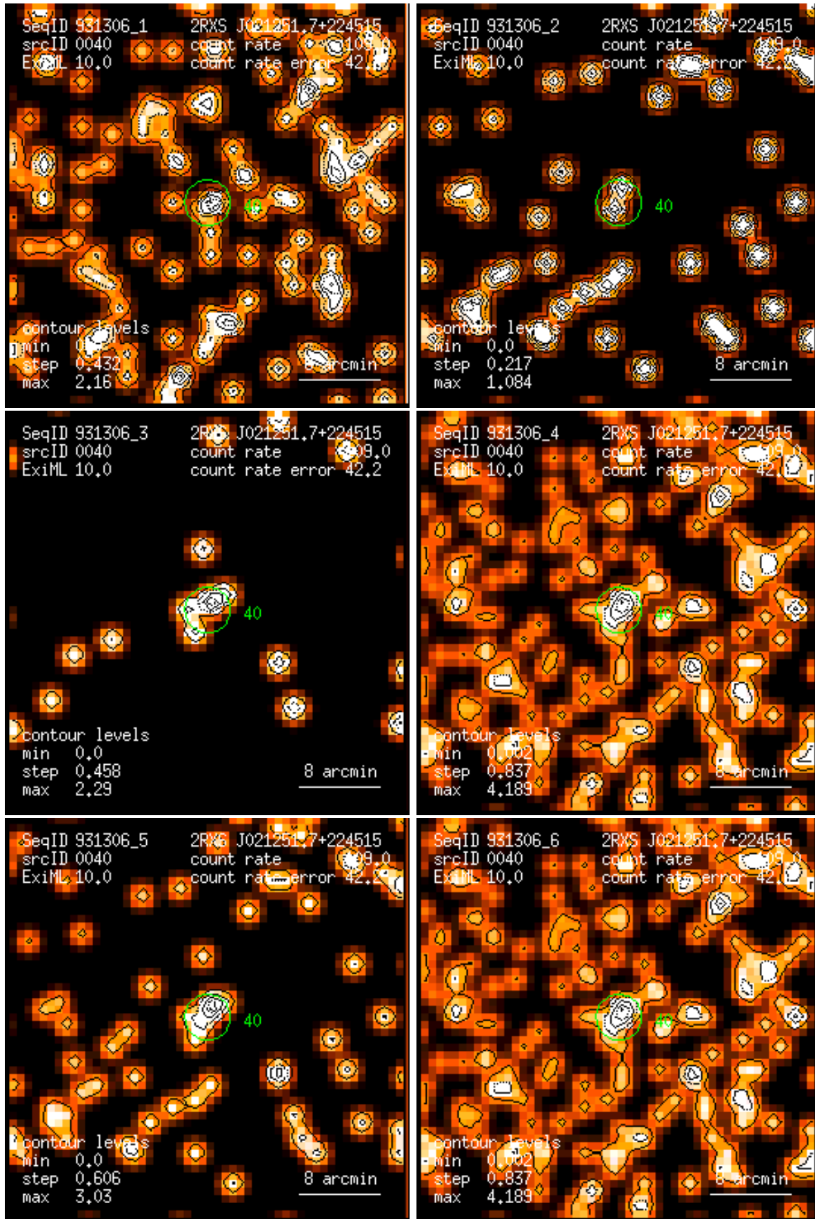
Figure 40: RASS 931306: detection 0040: band rate images, Gaussian filter: (1) PSPC channels 11 – 41, (2) 52 – 90, (3) 91 – 201, (4) 11 – 235, (5) 52 – 201, (6) 11 – 201. Broad band rates in counts/ks. Band rate contour levels in counts/ks/arcmin 2 .
