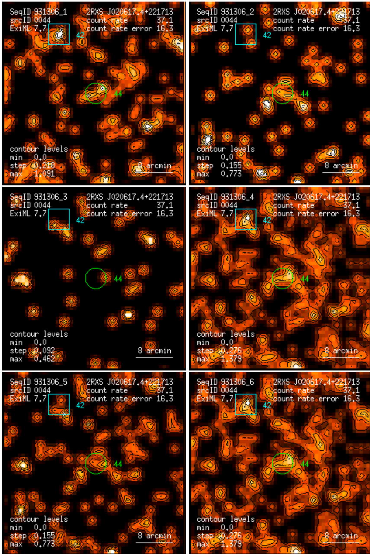
Figure 44: RASS 931306: detection 0044: band rate images, Gaussian filter: (1) PSPC channels 11 – 41, (2) 52 – 90, (3) 91 – 201, (4) 11 – 235, (5) 52 – 201, (6) 11 – 201. Broad band rates in counts/ks. Band rate contour levels in counts/ks/arcmin 2 .
