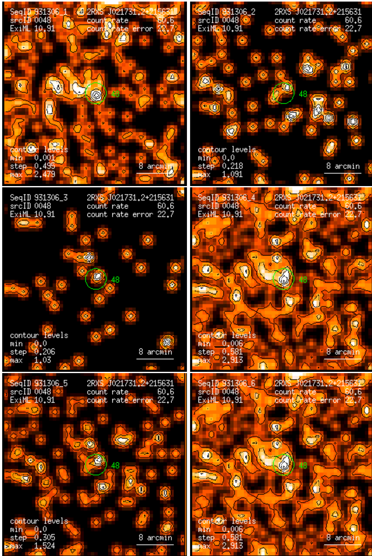
Figure 48: RASS 931306: detection 0048: band rate images, Gaussian filter: (1) PSPC channels 11 – 41, (2) 52 – 90, (3) 91 – 201, (4) 11 – 235, (5) 52 – 201, (6) 11 – 201. Broad band rates in counts/ks. Band rate contour levels in counts/ks/arcmin 2 .
