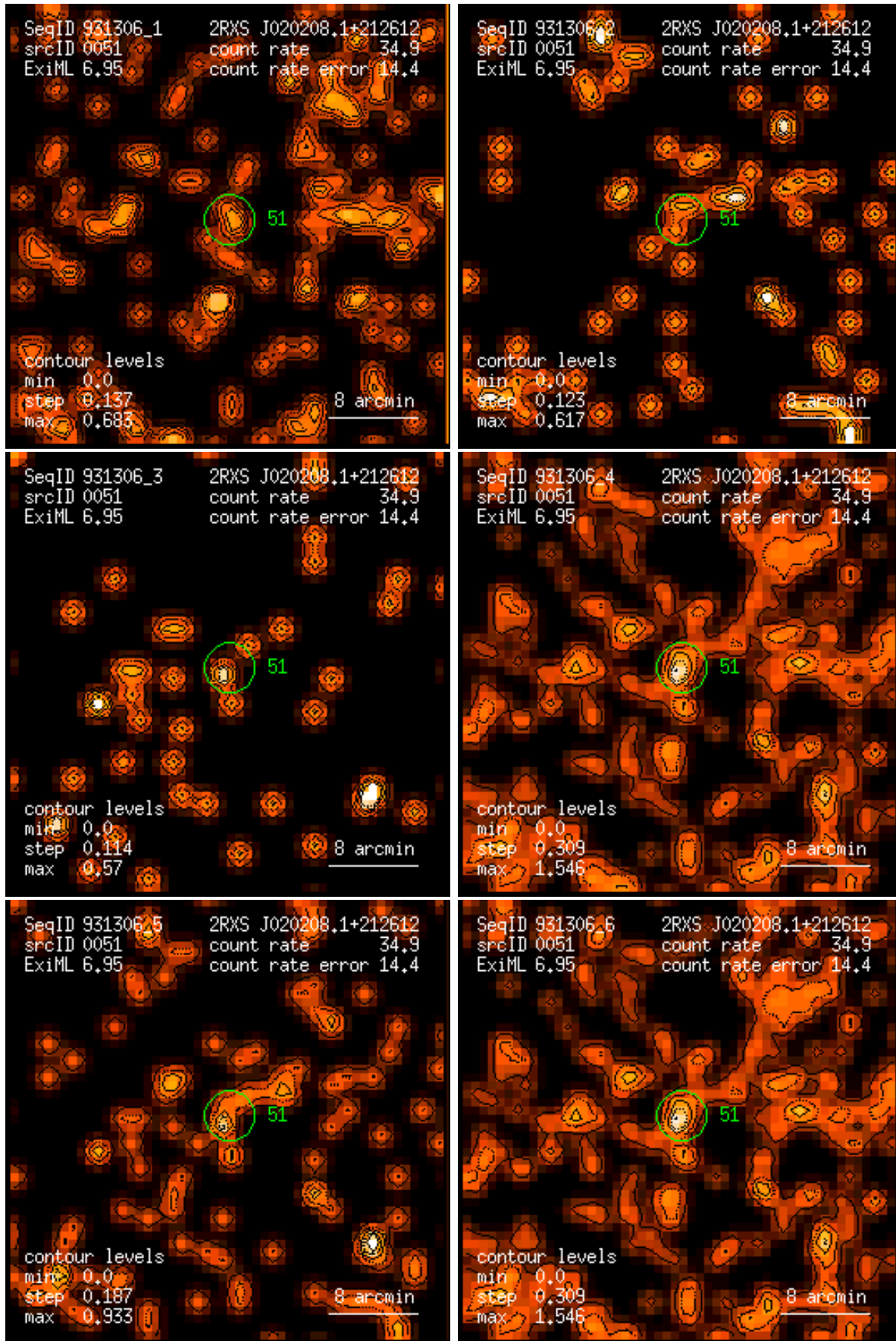
Figure 51: RASS 931306: detection 0051: band rate images, Gaussian filter: (1) PSPC channels 11 – 41, (2) 52 – 90, (3) 91 – 201, (4) 11 – 235, (5) 52 – 201, (6) 11 – 201. Broad band rates in counts/ks. Band rate contour levels in counts/ks/arcmin 2 .
