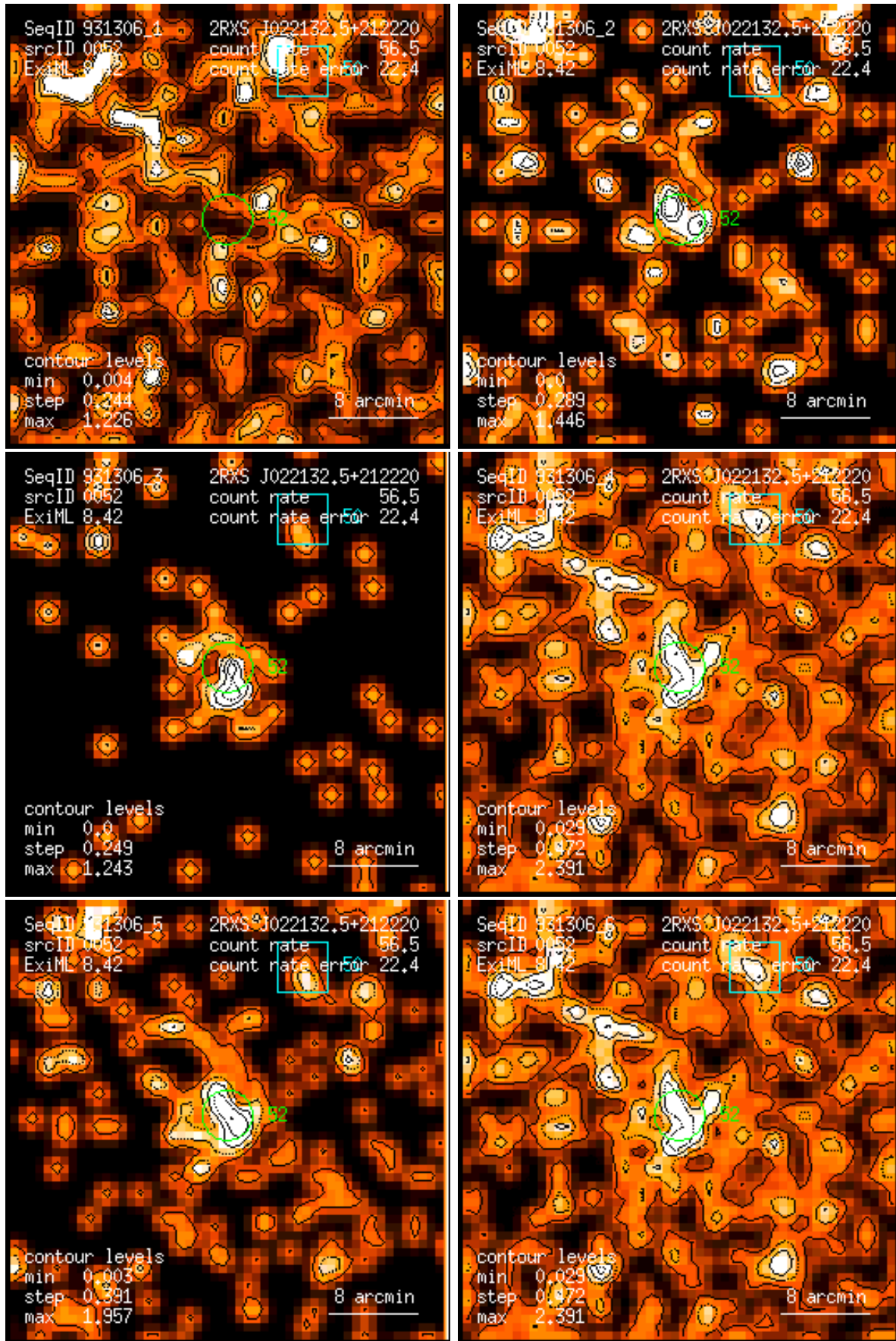
Figure 52: RASS 931306: detection 0052: band rate images, Gaussian filter: (1) PSPC channels 11 – 41, (2) 52 – 90, (3) 91 – 201, (4) 11 – 235, (5) 52 – 201, (6) 11 – 201. Broad band rates in counts/ks. Band rate contour levels in counts/ks/arcmin 2 .
