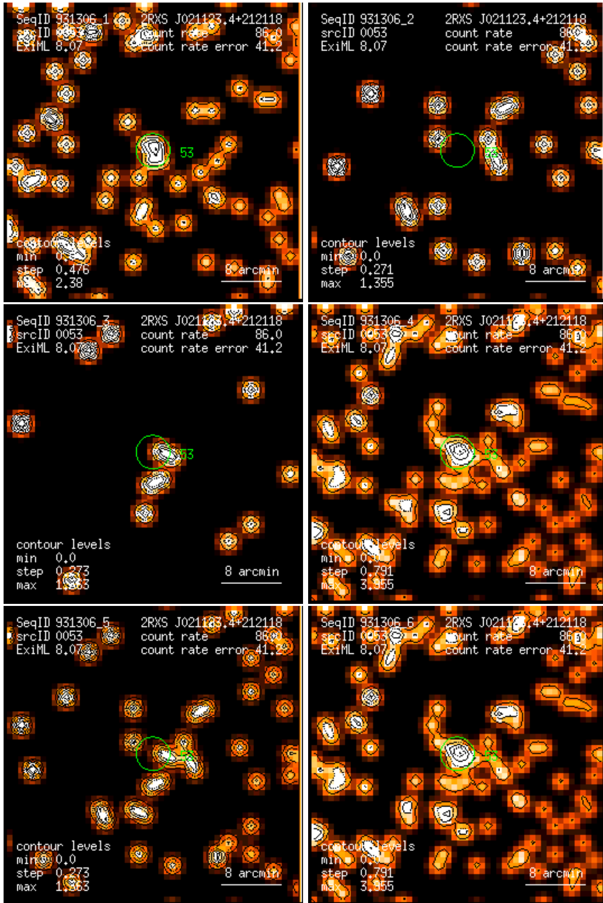
Figure 53: RASS 931306: detection 0053: band rate images, Gaussian filter: (1) PSPC channels 11 – 41, (2) 52 – 90, (3) 91 – 201, (4) 11 – 235, (5) 52 – 201, (6) 11 – 201. Broad band rates in counts/ks. Band rate contour levels in counts/ks/arcmin 2 .
