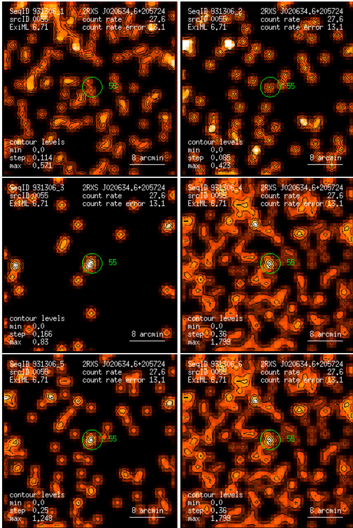
Figure 55: RASS 931306: detection 0055: band rate images, Gaussian filter: (1) PSPC channels 11 – 41, (2) 52 – 90, (3) 91 – 201, (4) 11 – 235, (5) 52 – 201, (6) 11 – 201. Broad band rates in counts/ks. Band rate contour levels in counts/ks/arcmin 2 .
