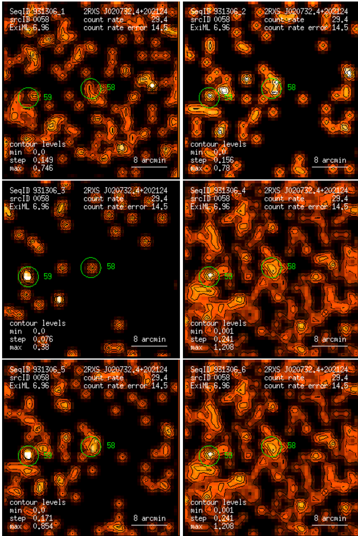
Figure 58: RASS 931306: detection 0058: band rate images, Gaussian filter: (1) PSPC channels 11 – 41, (2) 52 – 90, (3) 91 – 201, (4) 11 – 235, (5) 52 – 201, (6) 11 – 201. Broad band rates in counts/ks. Band rate contour levels in counts/ks/arcmin 2 .
