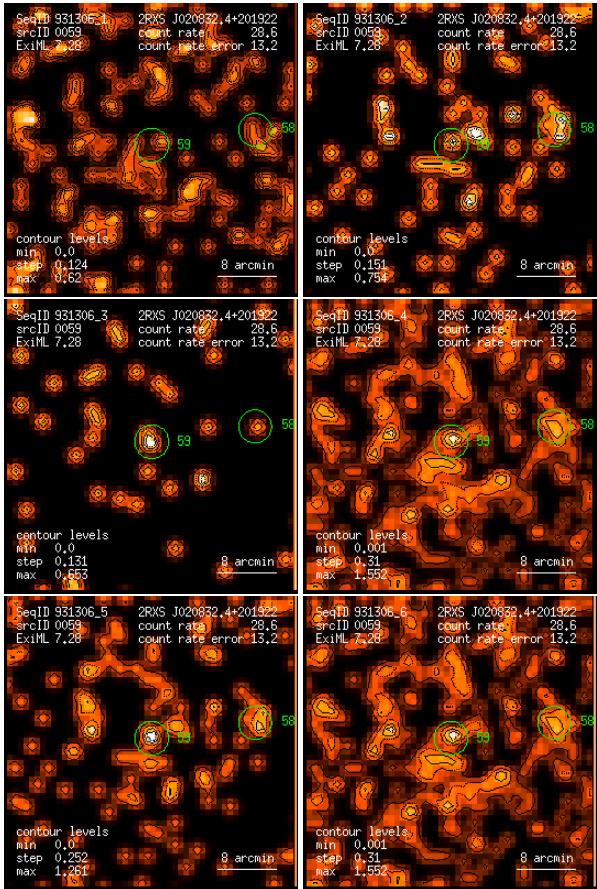
Figure 59: RASS 931306: detection 0059: band rate images, Gaussian filter: (1) PSPC channels 11 – 41, (2) 52 – 90, (3) 91 – 201, (4) 11 – 235, (5) 52 – 201, (6) 11 – 201. Broad band rates in counts/ks. Band rate contour levels in counts/ks/arcmin 2 .
