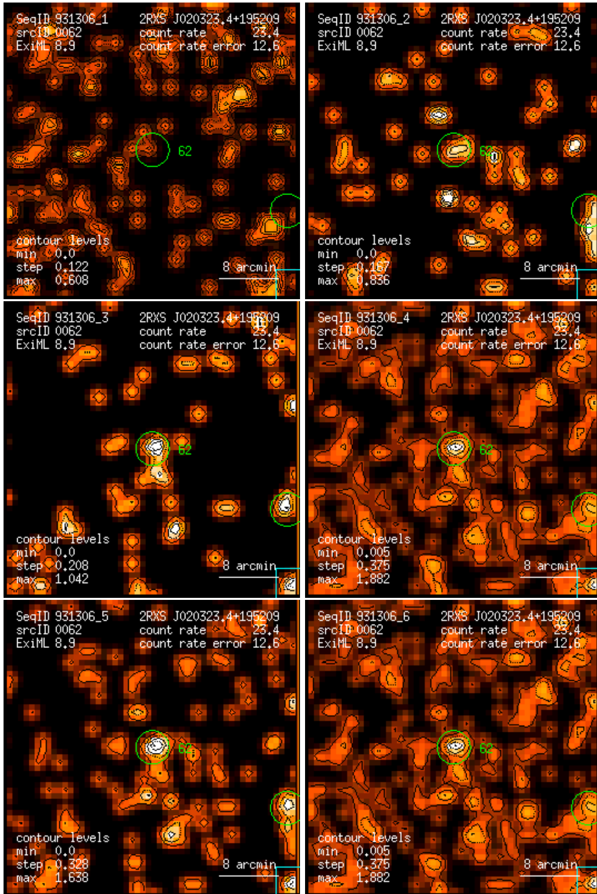
Figure 62: RASS 931306: detection 0062: band rate images, Gaussian filter: (1) PSPC channels 11 – 41, (2) 52 – 90, (3) 91 – 201, (4) 11 – 235, (5) 52 – 201, (6) 11 – 201. Broad band rates in counts/ks. Band rate contour levels in counts/ks/arcmin 2 .
