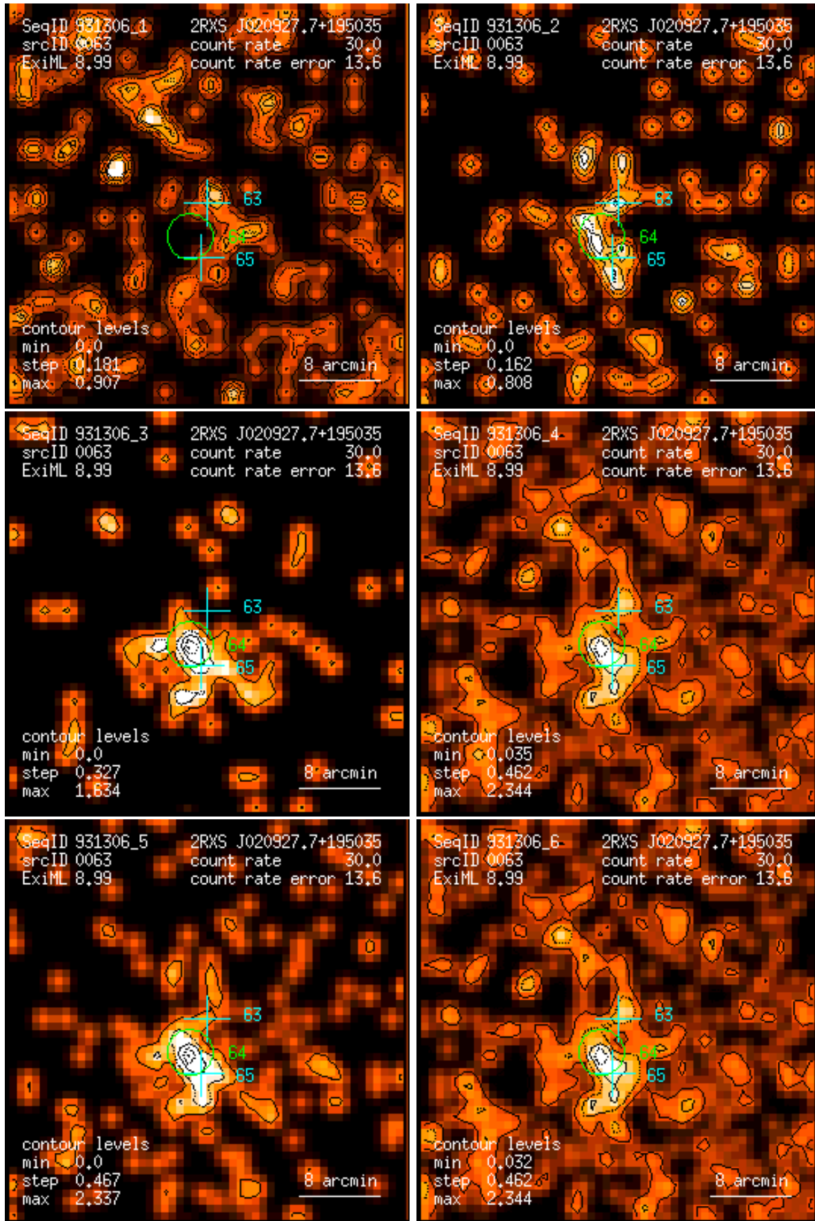
Figure 63: RASS 931306: detection 0063: band rate images, Gaussian filter: (1) PSPC channels 11 – 41, (2) 52 – 90, (3) 91 – 201, (4) 11 – 235, (5) 52 – 201, (6) 11 – 201. Broad band rates in counts/ks. Band rate contour levels in counts/ks/arcmin 2 .
