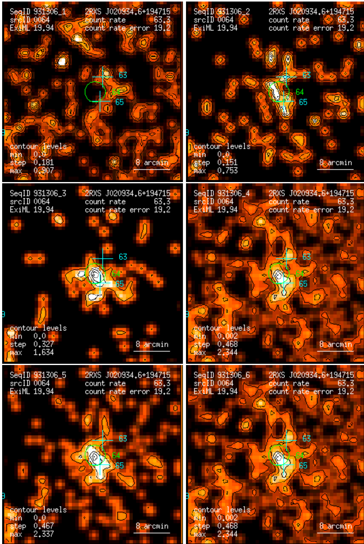
Figure 64: RASS 931306: detection 0064: band rate images, Gaussian filter: (1) PSPC channels 11 – 41, (2) 52 – 90, (3) 91 – 201, (4) 11 – 235, (5) 52 – 201, (6) 11 – 201. Broad band rates in counts/ks. Band rate contour levels in counts/ks/arcmin 2 .
