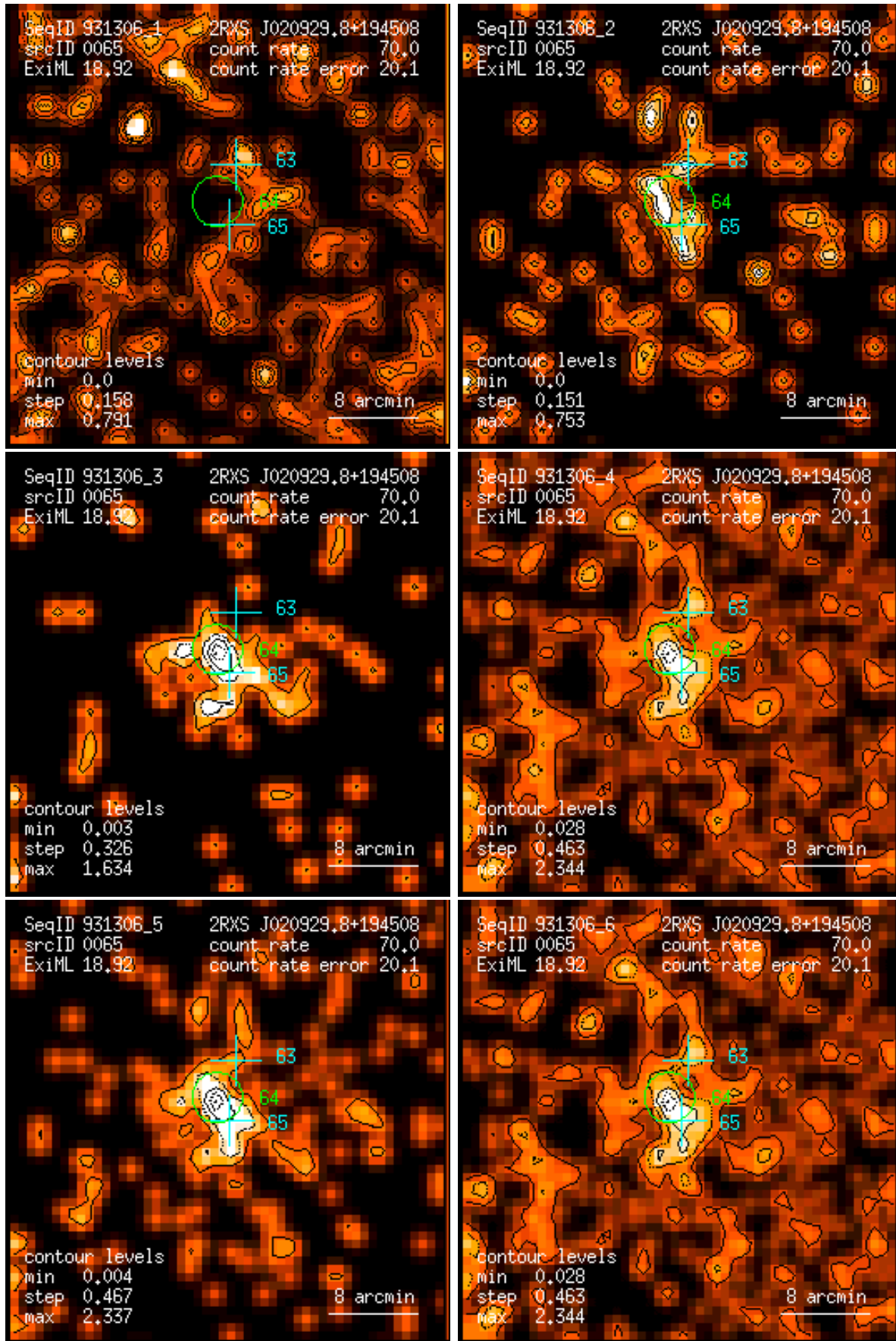
Figure 65: RASS 931306: detection 0065: band rate images, Gaussian filter: (1) PSPC channels 11 – 41, (2) 52 – 90, (3) 91 – 201, (4) 11 – 235, (5) 52 – 201, (6) 11 – 201. Broad band rates in counts/ks. Band rate contour levels in counts/ks/arcmin 2 .
