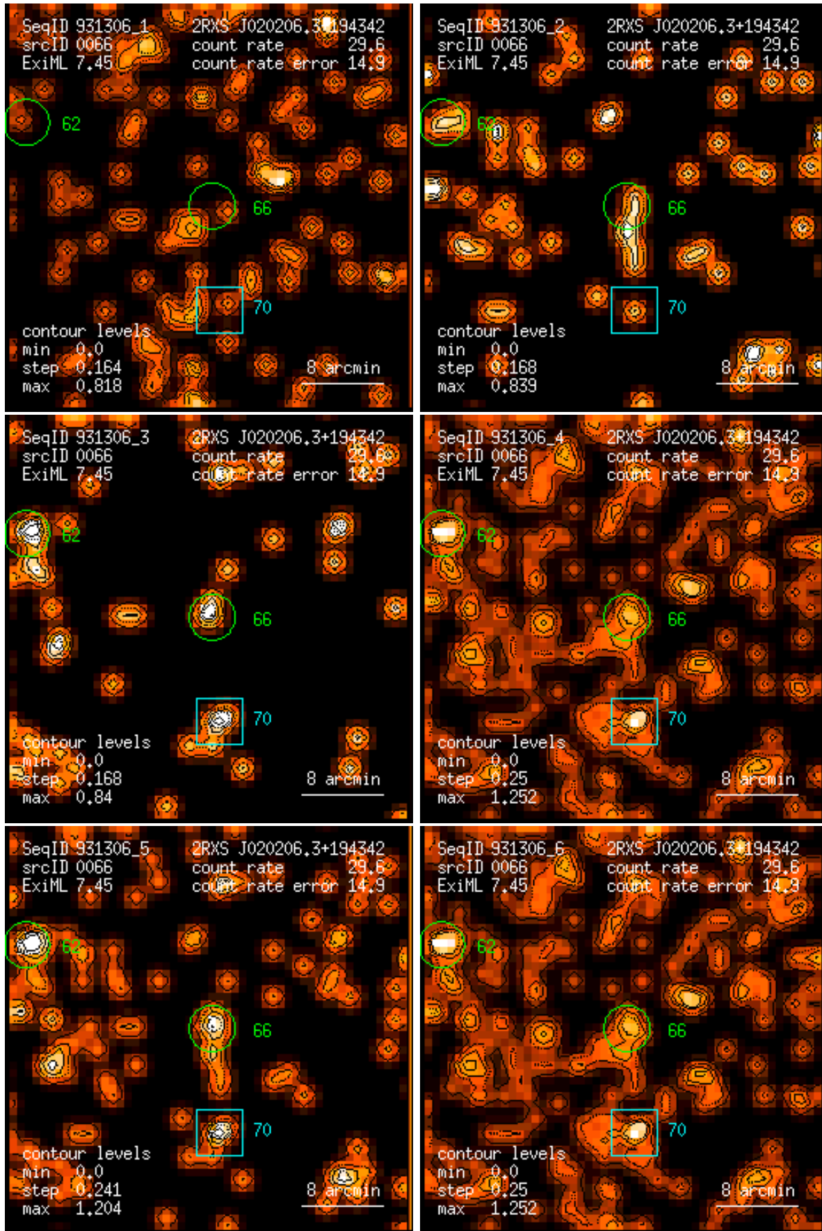
Figure 66: RASS 931306: detection 0066: band rate images, Gaussian filter: (1) PSPC channels 11 – 41, (2) 52 – 90, (3) 91 – 201, (4) 11 – 235, (5) 52 – 201, (6) 11 – 201. Broad band rates in counts/ks. Band rate contour levels in counts/ks/arcmin 2 .
