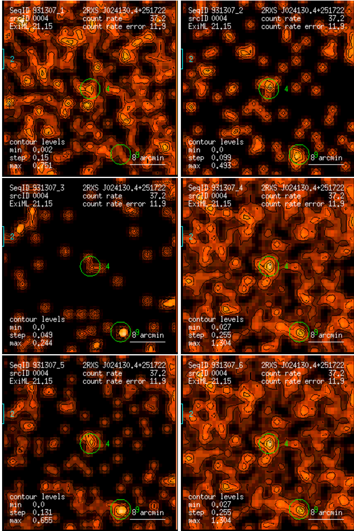
Figure 4: RASS 931307: detection 0004: band rate images, Gaussian filter: (1) PSPC channels 11 – 41, (2) 52 – 90, (3) 91 – 201, (4) 11 – 235, (5) 52 – 201, (6) 11 – 201. Broad band rates in counts/ks. Band rate contour levels in counts/ks/arcmin 2 .
