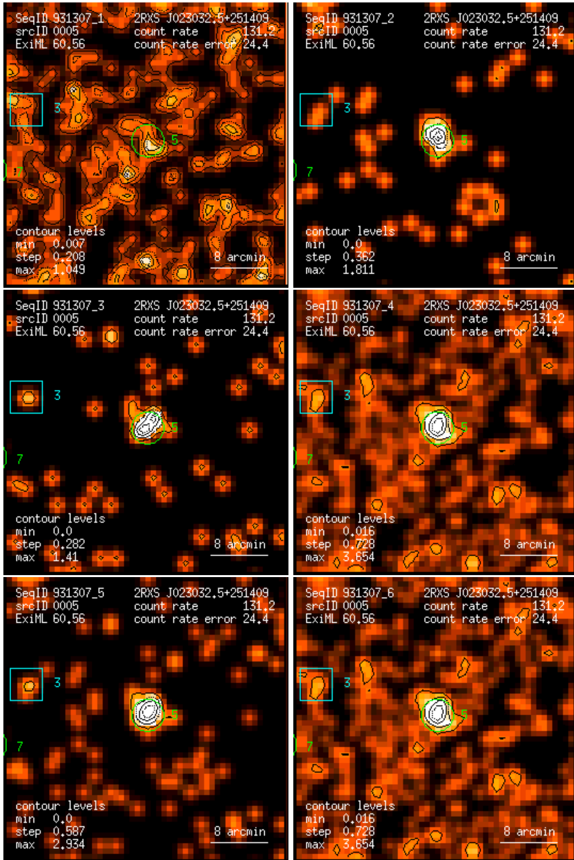
Figure 5: RASS 931307: detection 0005: band rate images, Gaussian filter: (1) PSPC channels 11 – 41, (2) 52 – 90, (3) 91 – 201, (4) 11 – 235, (5) 52 – 201, (6) 11 – 201. Broad band rates in counts/ks. Band rate contour levels in counts/ks/arcmin 2 .
