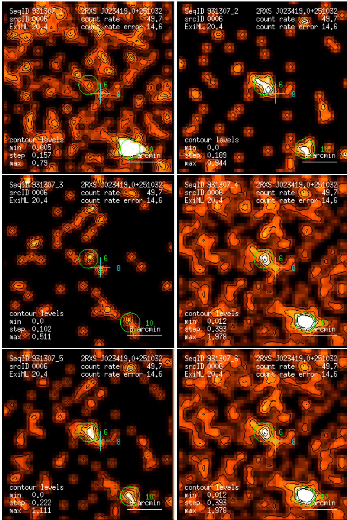
Figure 6: RASS 931307: detection 0006: band rate images, Gaussian filter: (1) PSPC channels 11 – 41, (2) 52 – 90, (3) 91 – 201, (4) 11 – 235, (5) 52 – 201, (6) 11 – 201. Broad band rates in counts/ks. Band rate contour levels in counts/ks/arcmin 2 .
