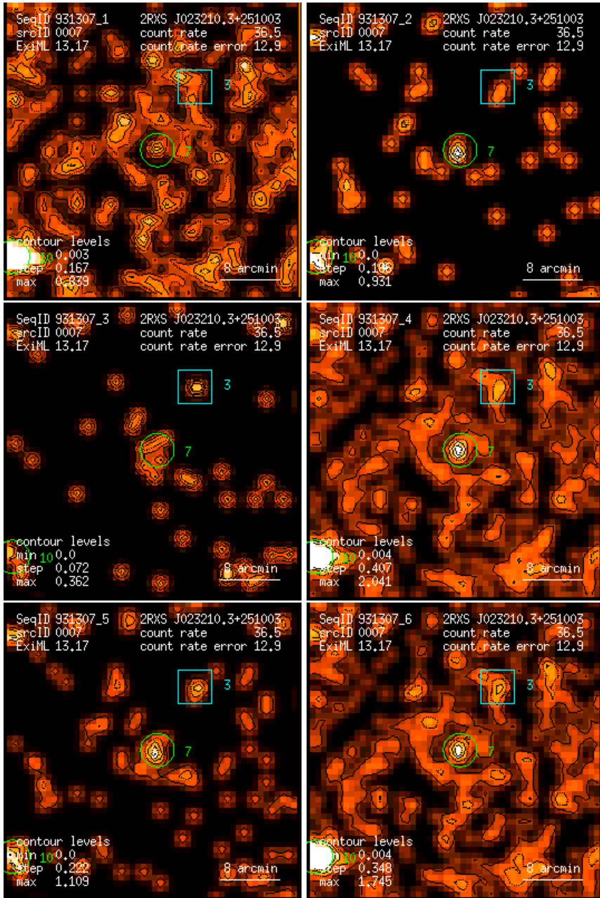
Figure 7: RASS 931307: detection 0007: band rate images, Gaussian filter: (1) PSPC channels 11 – 41, (2) 52 – 90, (3) 91 – 201, (4) 11 – 235, (5) 52 – 201, (6) 11 – 201. Broad band rates in counts/ks. Band rate contour levels in counts/ks/arcmin 2 .
