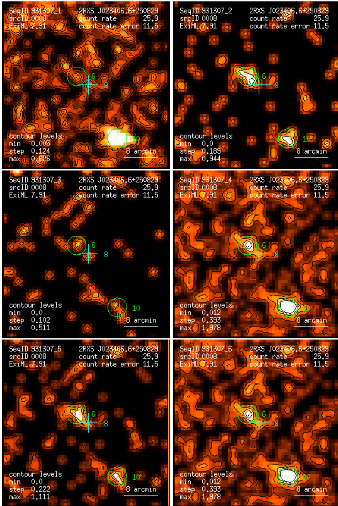
Figure 8: RASS 931307: detection 0008: band rate images, Gaussian filter: (1) PSPC channels 11 – 41, (2) 52 – 90, (3) 91 – 201, (4) 11 – 235, (5) 52 – 201, (6) 11 – 201. Broad band rates in counts/ks. Band rate contour levels in counts/ks/arcmin 2 .
