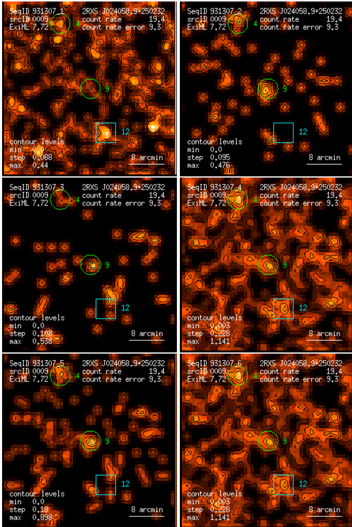
Figure 9: RASS 931307: detection 0009: band rate images, Gaussian filter: (1) PSPC channels 11 – 41, (2) 52 – 90, (3) 91 – 201, (4) 11 – 235, (5) 52 – 201, (6) 11 – 201. Broad band rates in counts/ks. Band rate contour levels in counts/ks/arcmin 2 .
