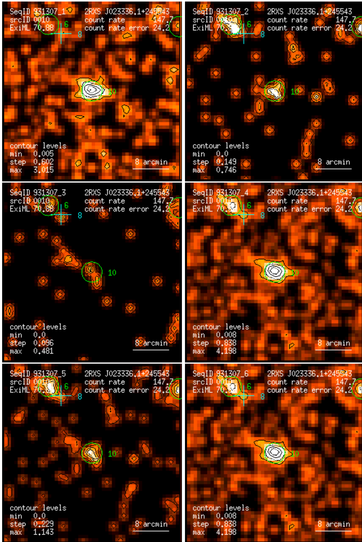
Figure 10: RASS 931307: detection 0010: band rate images, Gaussian filter: (1) PSPC channels 11 – 41, (2) 52 – 90, (3) 91 – 201, (4) 11 – 235, (5) 52 – 201, (6) 11 – 201. Broad band rates in counts/ks. Band rate contour levels in counts/ks/arcmin 2 .
