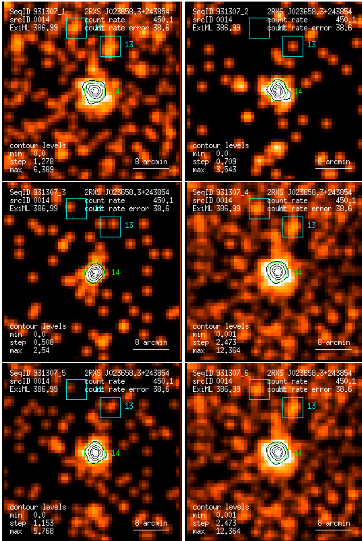
Figure 14: RASS 931307: detection 0014: band rate images, Gaussian filter: (1) PSPC channels 11 – 41, (2) 52 – 90, (3) 91 – 201, (4) 11 – 235, (5) 52 – 201, (6) 11 – 201. Broad band rates in counts/ks. Band rate contour levels in counts/ks/arcmin 2 .
